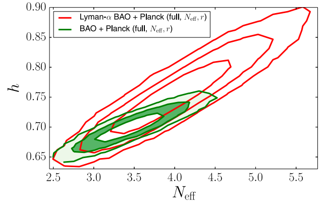
FIG. 17 (color online). Constraints on the effective number of relativistic species N_{\text{eff}} , assuming w = -1 and \Omega_k = 0 . These contours use full Planck + WP CMB constraints computed with COSMOMC, combined with Ly \alpha F BAO only (red) or with our full set of BAO measurements (green). We marginalize over the tensor-to-scalar ratio r .
