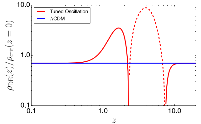
FIG. 19 (color online). Implied variation in the energy density of the dark energy component for the model shown in Fig. 18. The dotted line corresponds to the density becoming negative. These plots illustrate the difficulty of concurrently fitting the Ly \alpha F and galaxy BAO constraints on D_M and D_H while satisfying the CMB constraint on D_M .
