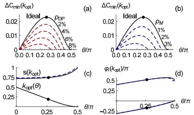
FIG. 2. (a) Maximum violation of the modified Helstrom bound as a function of the state-separation angle \theta . The ideal violation (solid line) is reduced in the presence of depolarization decoherence with strength p_{\text{DP}} increasing in increments of 2%. (dashed lines). (b) The ideal violation (solid line) is similarly reduced in the presence of measurement misidentification errors with probability p_M increasing in increments of 1%. (c) Lower curve: the optimal cost parameter k_{\text{opt}}(\theta) for the maximum MH bound violation [Eq. (9), peaks in Fig. 1(c)] in the ideal case. Upper curves: the optimal measurement strength s for the cascaded partial measurement scheme, as a function of \theta , for the optimal cost parameter k_{\text{opt}}(\theta) . (d) Optimal angles \varphi_1 (lower curves) and \varphi_2 (upper curves) for the cascaded partial measurement scheme. In both (c) and (d) the solid curves are for the ideal case, while the (almost identical) dashed curves include 2% misidentification noise. The black dots indicate the globally maximum ideal violation.
