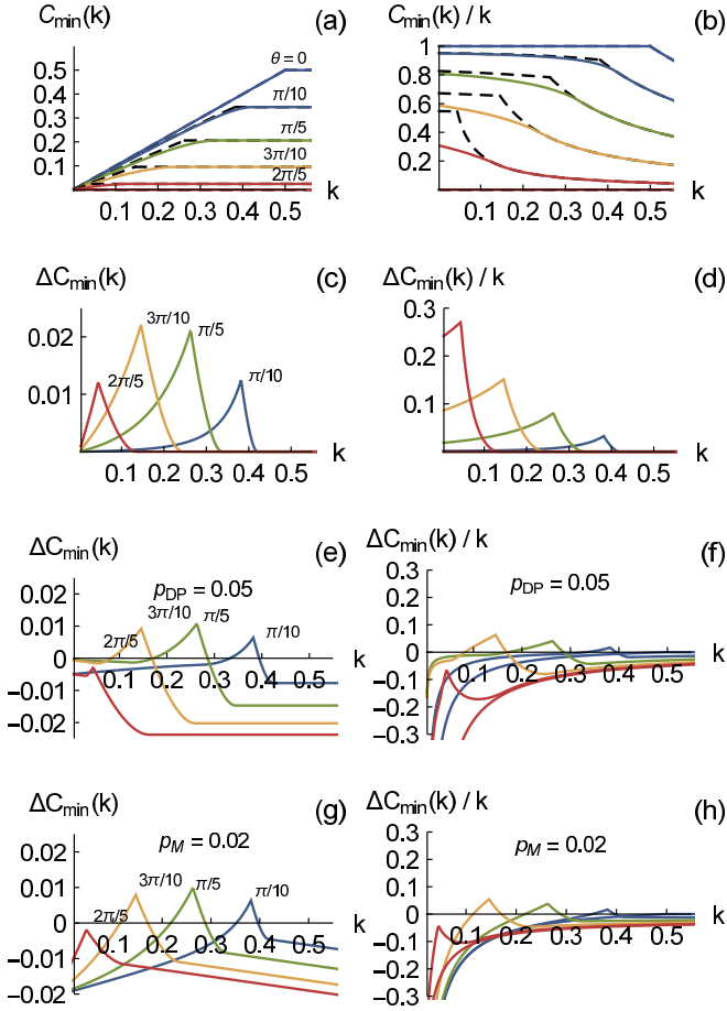
FIG. 1. (a) Minimum cost for discriminating |\psi_0\rangle = |0\rangle and |\psi_1\rangle = \cos\theta|0\rangle + \sin\theta|1\rangle by a measurement, using the cost function C(k) = p_w + k p_d to penalize wrong, p_w , and declined, p_d , guess probabilities. Shown are separation angles \theta in increments of \pi/10 . Dashed lines show the modified Helstrom bound C_{\text{MH}} , Eq. (8), attainable with a projective measurement, with the horizontal part being the usual Helstrom bound. Solid lines (same colors in all panels) show the minimum cost C_{\text{min}} for nonprojective measurements, and violate the MH bound for a range of k . (b) Same as in (a) for the scaled cost function C(k)/k . This scaling permits the case of unambiguous state discrimination to be recovered at k \rightarrow 0 . (c) Violation of the MH bound, \Delta C_{\text{min}} = C_{\text{MH}} - C_{\text{min}} , showing the difference between the dashed and solid curves in (a). (d) Violation of the scaled bound, \Delta C_{\text{min}}/k . (e) and (f) Same as (c,d) but with 5% probability p_{\text{DP}} of depolarizing the states. (g) and (h) Same as (c,d) but with 2% probability p_{\text{M}} of misidentifying the measured result. These imperfections increase C_{\text{min}} and therefore decrease the violation \Delta C_{\text{min}} . Note that for the USD case [ k \rightarrow 0 in (f) and (h)] the cost advantage is fully destroyed by experimental imperfections, but the MH bound violation is still possible for intermediate k .
