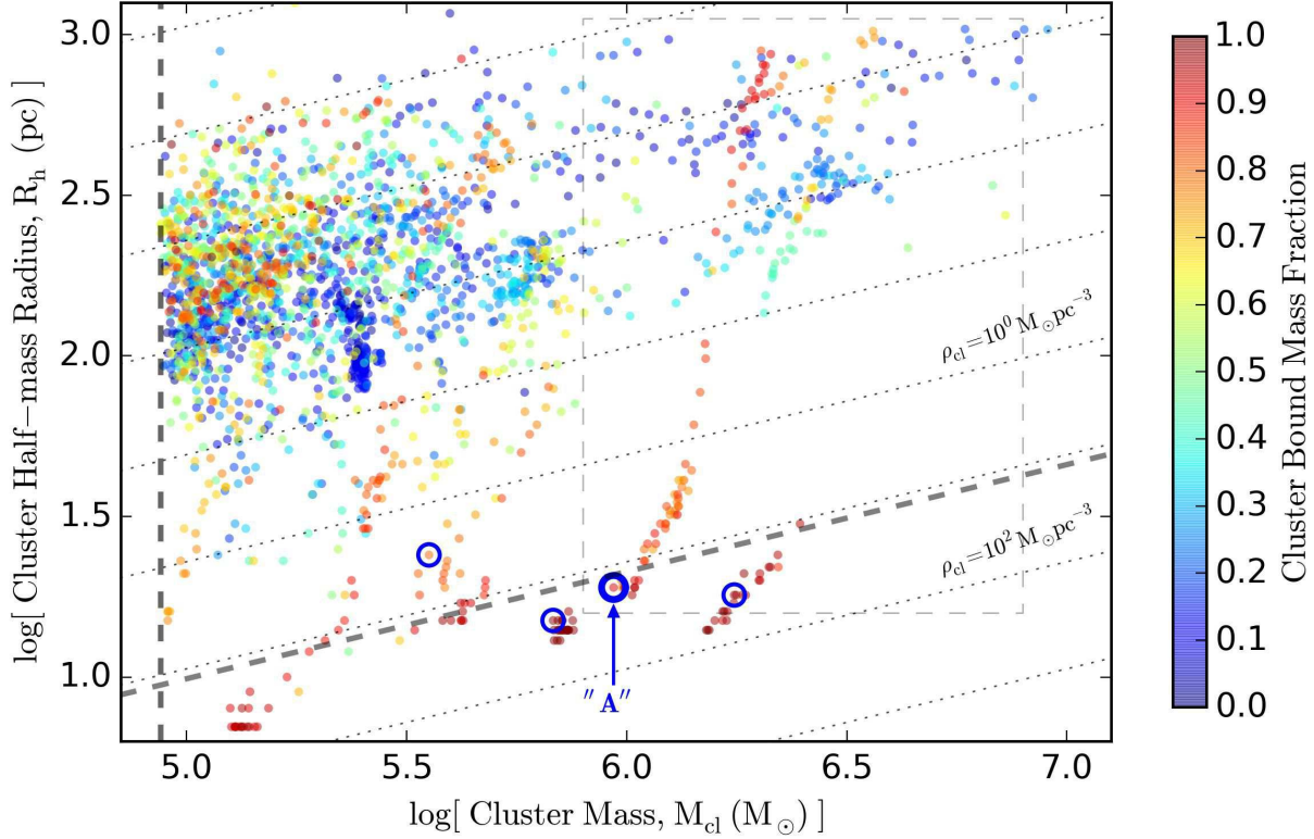
Figure 4. Cluster mass, M_{\text{cl}} , versus half-mass radius, R_{\text{h}} for all star clusters identified by ROCKSTAR in all 76 snapshots finely spaced between z = 7 and z = 5 , that survived at least one output interval (e.g., \Delta t_{\text{out}} \sim 1.6 Myr at 6.5 < z < 7 ; see footnote 5). Each data point is colored by the fraction of member particle masses that are bound to the cluster center, f_{\text{bd}} . The cluster “A” from Figures 1-3 is marked with a thick blue circle at z = 5 . Three other thin blue circles indicate the other long-lasting bound clusters identified at z = 5 . For references, the thin dotted diagonal lines denote the slope of constant stellar density, while the thick dashed diagonal line marks the star formation threshold density, 500 \text{ cm}^{-3} or 12 M_{\odot} \text{ pc}^{-3} . The thick dashed vertical line represents the threshold mass to be identified as a star cluster, 8.74 \times 10^4 M_{\odot} . Most of the objects are young, loose associations with stellar densities \sim 10^{-2} M_{\odot} \text{ pc}^{-3} and little bound mass (upper left corner). The few low-density associations with high bound mass fraction represent systems with a bound core and a loosely-bound “envelope” (upper right corner). They rapidly evolve to become more dense clusters (blue circles; see Figure 7 for more information that zooms in on the gray dashed rectangular region).
