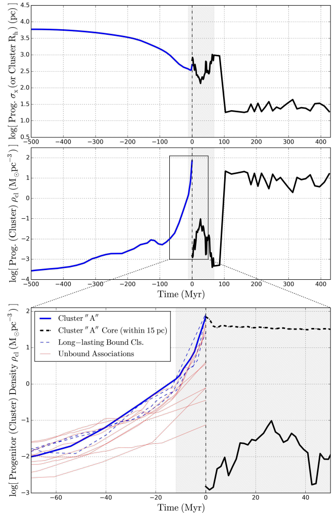
Figure 9. Evolution of the cluster “A” and its gas progenitor. Top: the gas progenitor member particles’ dispersion in position, \sigma (blue), or the cluster’s half-mass radius, R_{\text{h}} (black; corresponding to the y-axis of Figure 7). A vertical dot-dashed line in each panel marks 0 Myr, the moment the cluster forms. The gray shaded region shows the period in which the simulation produced outputs at finer intervals. Middle: the gas progenitor member particles’ mean density, \bar{\rho}_{\text{gas}} (blue), or the cluster’s mean stellar density, \rho_{\text{cl}} \equiv 3M_{\text{cl}}/(8\pi R_{\text{h}}^3) (black). Triggered by a galaxy merger, the gas progenitor’s density increases in a short time, causing the gas cloud to collapse and turn a significant portion of its mass, \gtrsim 10^5\text{--}6 M_{\odot} , simultaneously into stars. Bottom: a zoom-in region around the cluster formation time. The discontinuity in densities between the blue and black solid lines at 0 Myr is because the newly-formed star cluster grouped by ROCKSTAR includes not only the just born star particles but also nearby pre-existing stars and the low-density “envelope” of stars forming from nearby less dense gas. But the gas progenitor’s density smoothly transitions to the cluster’s core density within 15 pc from its center (thick black dashed line) that contains almost exclusively newly-born star particles. In addition to the gas progenitor of the cluster “A” (thick blue line), progenitors of three other long-lasting bound clusters identified at z = 5 are shown (blue dashed lines). Also shown are the progenitors of nine unbound associations at z = 5 – that are more massive than 1.5 \times 10^5 M_{\odot} at z = 5 , but did not become long-lasting bound clusters (thin red lines). All the bound clusters follow a similar evolutionary path, with a large mass collectively reaching high densities in a short timescale ( \sim 10 Myr). Unbound associations typically form from fragmenting sub-regions within lower-mean-density GMC complexes.
