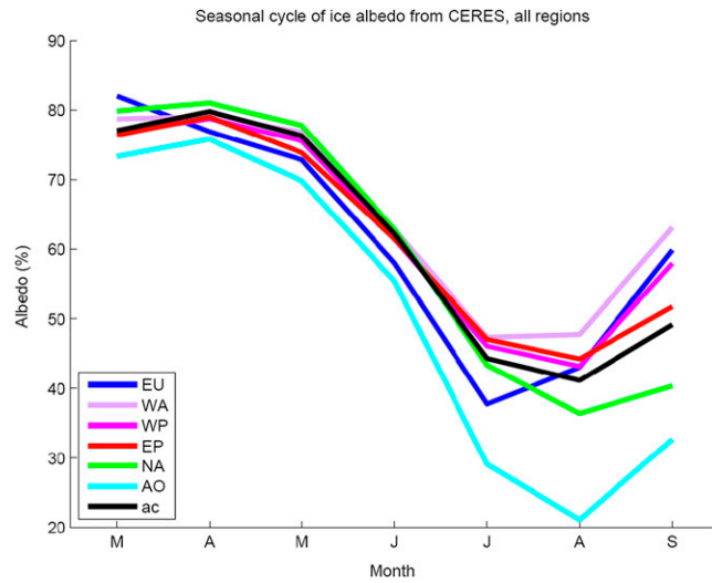
Fig. 55. Seasonal cycle of sea ice surface albedo based on CERES data from each region. Note that all regions have a similar seasonal cycle, although the AO and EU regions differ somewhat from the other four regions, which is consistent with these being the two regions with the smallest amount of ice and hence requiring the largest extrapolation to ascertain the albedo associated with 100% ice cover.
