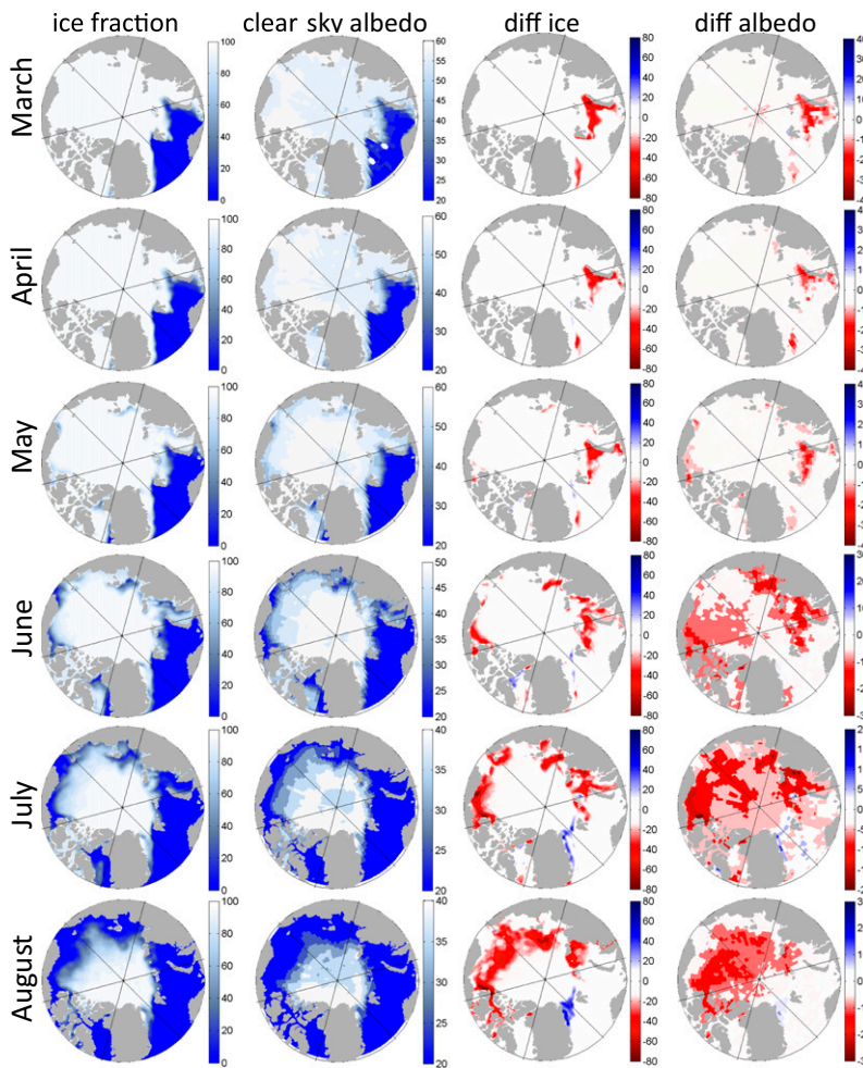
Fig. S1. As in Fig. 1, but for the months March through August: ( Far Left ) Special Sensor Microwave Imager (SSM/I) sea ice concentration and ( Middle Left ) CERES clear-sky albedo averaged over the last 5 y of the CERES record (2007–2011), and ( Middle Right ) change in sea ice and ( Far Right ) change in clear-sky albedo between the last 5 y (2007–2011) and the first 5 y (2000–2004) of the CERES record. Note the agreement between sea ice and planetary albedo.
