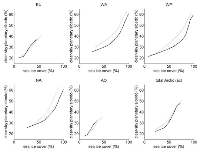
Fig. S4. As in Fig. 2, but for the other regions defined in Fig. S2 as well as for the total Arctic. Note that CCSM4 gives results fairly similar to CERES, although the change in slope occurring around June is less pronounced in the model output, and the model gives a higher summer minimum albedo.
