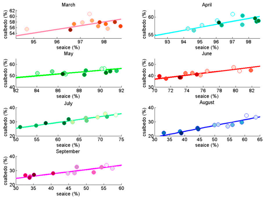
Fig. 56. As in Fig. 2, but for each month individually to indicate the linear fits to the data (solid lines) used to produce Fig. 4.
