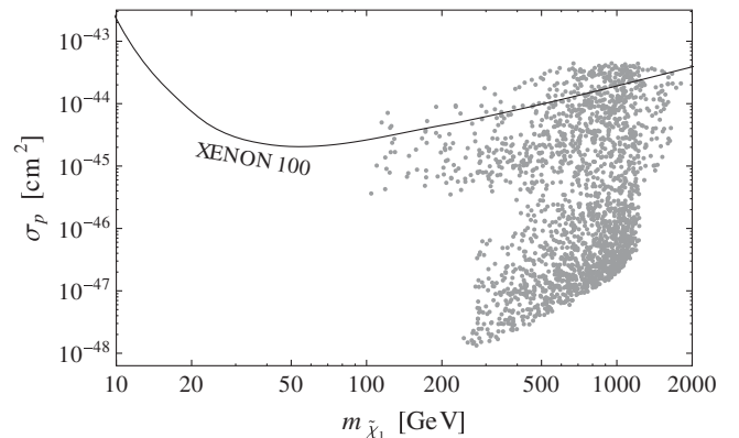
FIG. 7. Neutralino proton cross section for the benchmark points with successful gauge coupling unification (gray). The current limit from the XENON100 direct dark matter search is also shown. The latter is only applicable if the lightest neutralino accounts for all dark matter in the Universe.
