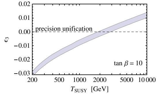
FIG. 1 (color online). Deviation from PGU as a function of T_{\text{SUSY}} . The width of the band corresponds to the 1\sigma experimental error in \alpha_s(M_Z) .
