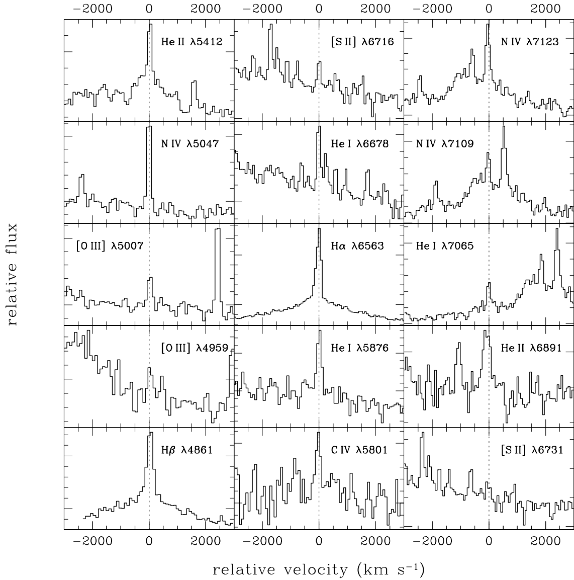
Figure 2: Emission-line velocity structure at 15.5 hr. The strongest lines ( H\alpha and H\beta , He II \lambda 5411 , and the N IV \lambda 7115 complex) show broad wings extending out to \sim 2500 \text{ km s}^{-1} . Other weaker lines are narrow and unresolved.
