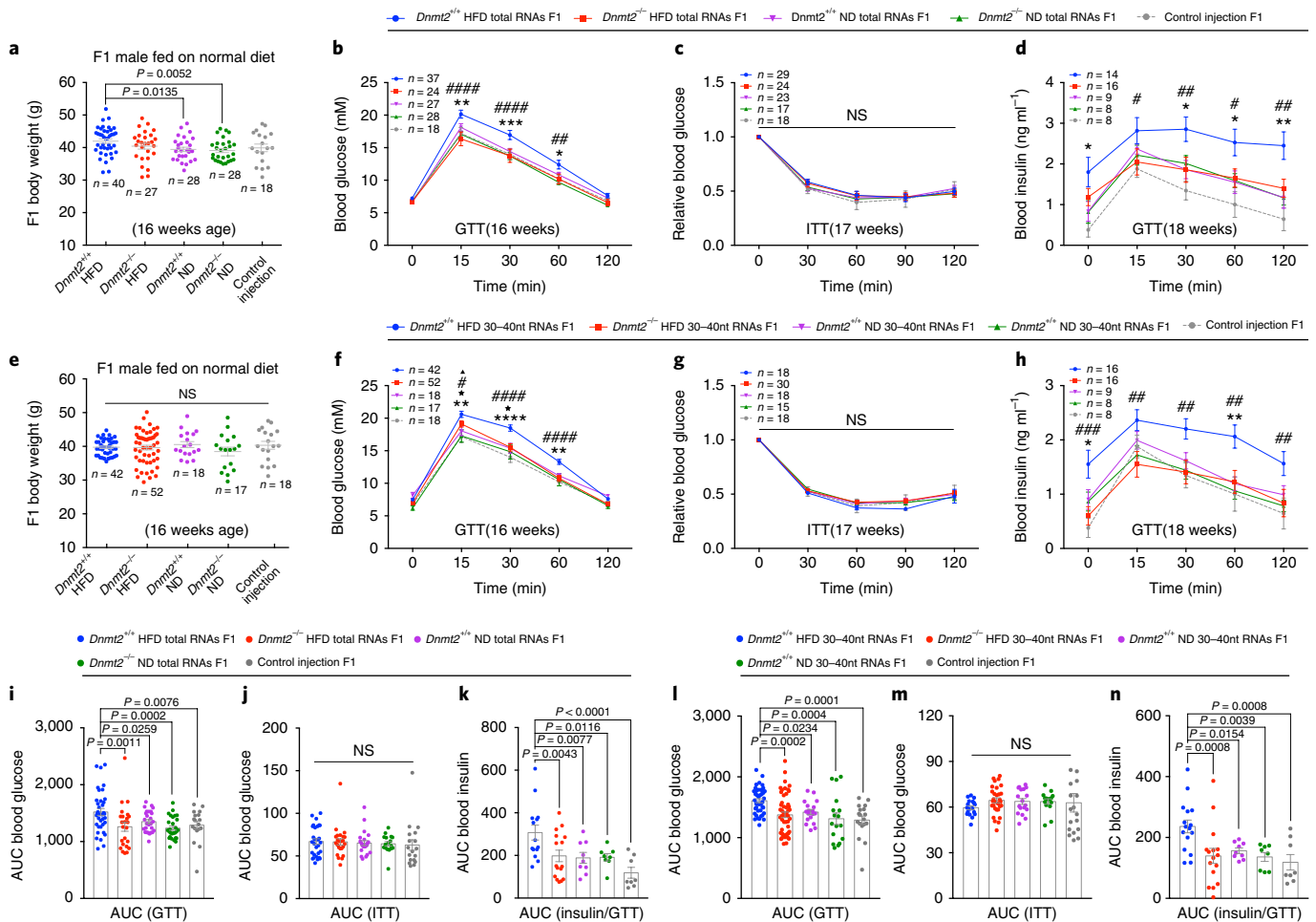
Fig. 2 | Body weight and metabolic parameters of F1 males generated by zygotic injection of sperm total RNAs or 30–40 nt RNAs, fed on a ND. a–d , Body weight and metabolic phenotypes of F1 males generated from injection of sperm total RNAs: body weight ( a ); blood glucose during GTT ( b ); relative blood glucose during ITT ( c ); serum insulin during GTT ( d ). n = number of mice in each group. In a , each dot represents one mouse; data are pooled from 10 experiments. In b , data are pooled from 10 experiments; * P < 0.05, ** P < 0.01, *** P < 0.001 ( Dnmt2 +/+ HFD F1 versus Dnmt2 +/+ ND F1); ### P < 0.01, #### P < 0.0001 ( Dnmt2 +/+ HFD F1 versus Dnmt2 -/- HFD F1). In c , data are pooled from eight experiments. NS, not significant. In d , data are pooled from seven experiments; * P < 0.05, *** P < 0.01 ( Dnmt2 +/+ HFD F1 versus Dnmt2 +/+ ND F1); # P < 0.05, ## P < 0.01 ( Dnmt2 +/+ HFD F1 versus Dnmt2 -/- HFD F1). i–k , AUC statistics for b,c,d , respectively. NS, not significant. e–h , Body weight and metabolic phenotypes of F1 males generated from sperm 30–40 nt RNAs injection: body weight ( e ); blood glucose during GTT ( f ); relative blood glucose during ITT ( g ); serum insulin during GTT ( h ). In e , each dot represents one mouse, and data are pooled from 10 experiments; NS, not significant. In f , data are pooled from 10 experiments; ** P < 0.01, **** P < 0.0001 ( Dnmt2 +/+ HFD F1 versus Dnmt2 +/+ ND F1); # P < 0.05, #### P < 0.0001 ( Dnmt2 +/+ HFD F1 versus Dnmt2 -/- HFD F1); ▲ P < 0.05 ( Dnmt2 -/- HFD F1 versus Dnmt2 -/- ND F1); * P < 0.05 ( Dnmt2 -/- HFD F1 versus control injection F1). In g , data are pooled from seven experiments; NS, not significant. In h , data are pooled from seven experiments; * P < 0.05, ** P < 0.01 ( Dnmt2 +/+ HFD F1 versus Dnmt2 +/+ ND F1); ## P < 0.01, ### P < 0.001 ( Dnmt2 +/+ HFD F1 versus Dnmt2 -/- HFD F1). i,m,n , AUC statistics for f,g,h , respectively; NS, not significant. All data are plotted as mean ± s.e.m. Statistical analyses were performed by two-tailed, one-way ANOVA ( a,e,i–n ) or two-way ANOVA ( b–d,f–h ), uncorrected Fisher’s LSD. NS, not significant. All statistic source data and P values are provided in Supplementary Table 1.
