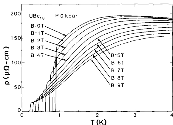
Fig 1 Resistivity versus temperature for UBe_{13} at zero pressure and at the magnetic field values indicated
