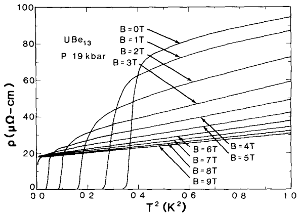
Fig 4 Resistivity versus temperature-squared for UBe_{13} at 19 kbar and at the magnetic field values indicated
