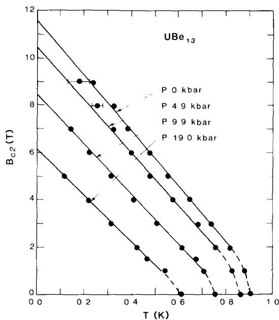
Fig 3 Upper critical magnetic field versus temperature for UBe_{13} at the pressure values indicated. The lines are only a guide to the eye.
