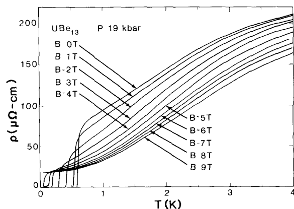
Fig 2 Resistivity versus temperature for UBe_{13} at 19 kbar and at the magnetic field values indicated
