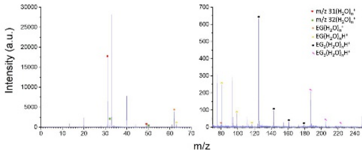
Figure 1 40% EG mass spectrum recorded at 12.0 eV. The cluster series for m/z 31(\text{H}_2\text{O})_n^+ , m/z 32(\text{H}_2\text{O})_n^+ , m/z 62(\text{H}_2\text{O})_n^+ , m/z 63(\text{H}_2\text{O})_n^+ , m/z 125(\text{H}_2\text{O})_n^+ , and m/z 187(\text{H}_2\text{O})_n^+ are indicated with colored dots. Ethylene glycol has a mass of 62 amu.
