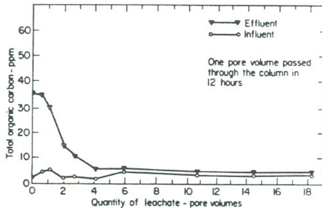
Figure 6. Progressive decrease in leachate strength - all organic carbon is leached by first six pore volumes. XBL 791-246
