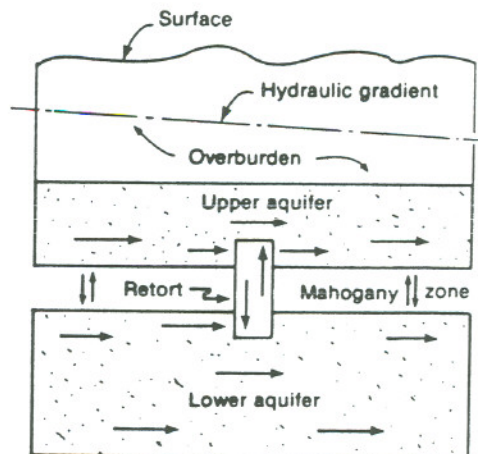
Figure 1. Schematic of retort-aquifer configuration in Piceance Basin. XBL 786-994
