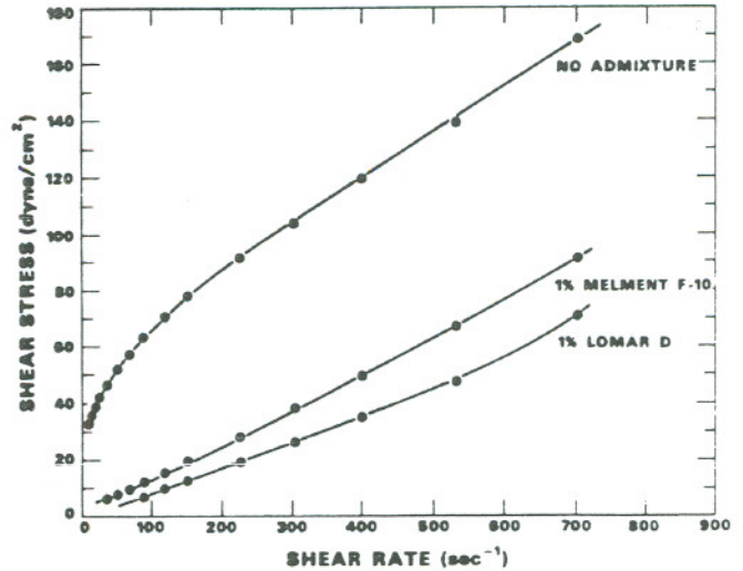
Figure 3. Viscosity-reducing effect of admixtures on spent shale slurries (45% solids). XBL 794-1187
