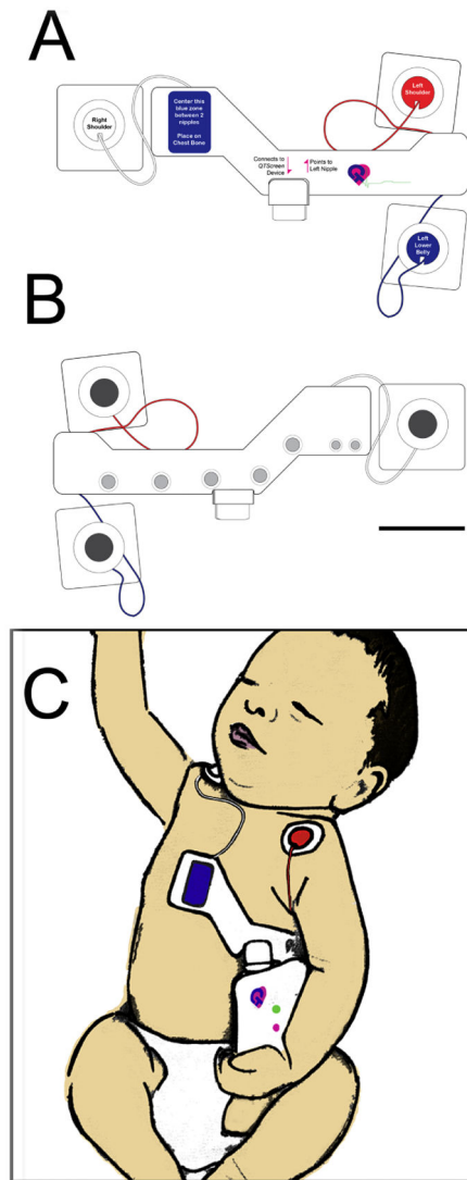
Fig. 1. Drawings of the one-piece ECG electrode strip, made of flexible printed circuit boards (FPCBs) sandwiched between non-woven fabric (top surface) and a thin layer of medical foam material with 3M adhesive (on the undersurface, for skin contact). Three limb electrodes extend from the ends of the strip -- 2 from the left end for the LA (red circle) and LL electrodes (blue circle), and one from the right end for the RA electrode (white circle). A. Top surface, showing the snap-on connector for the ECG recorder and instructions for placing the strip. B. Undersurface, showing 7 Ag/AgCl hydrogel sensors for the chest and RL electrodes (5 or 8 mm in diameter). Each of the 3 wires for the limb electrodes is connected to an adhesive circle with an Ag/AgCl hydrogel sensor (10 mm in diameter). Scale bar = 4 cm. C. A correctly placed electrode strip, with the ECG recorder attached and functioning. The infant pictured is 3 weeks old.
