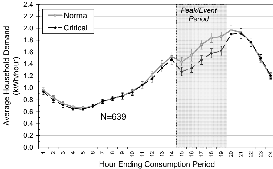
Figure 5. Hourly usage on normal and critical days during hot weather, 95-104.9°F
