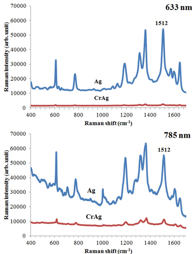
Figure 9 | SERS spectra obtained from Rhodamine 6G dropped onto structured areas coated with only Ag (60 nm), or Cr (5 nm) and Ag (60 nm) layers using 633 nm (800 nm void size) and 785 nm (1400 nm void size) lasers.
