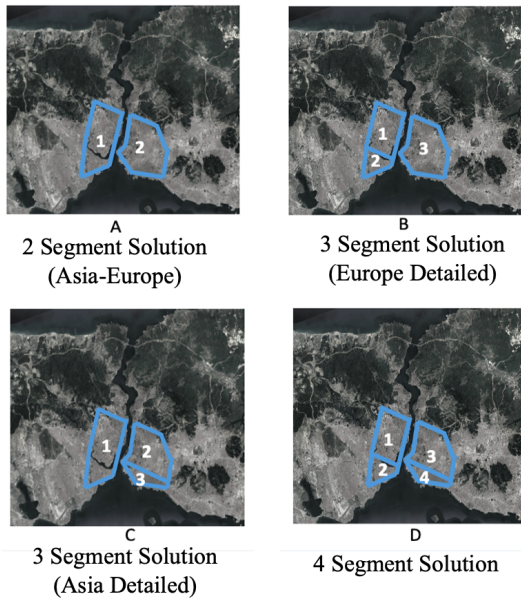
Figure 1: Four segmentation options.
