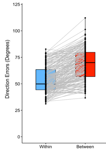
Figure 5: Within segment and between segment direction errors.
