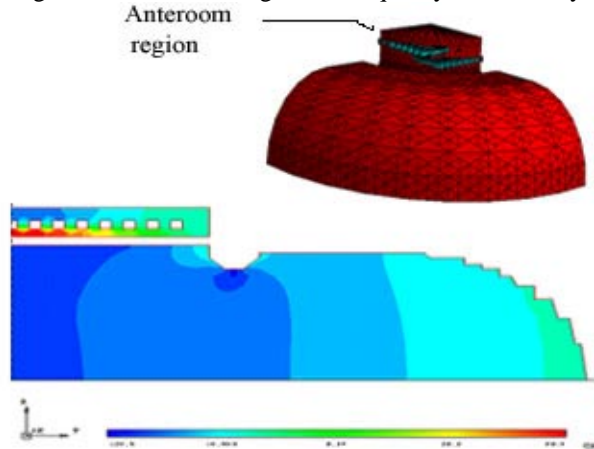
Figure 5: E_z field for case 1 15 x 15 array, grids not touching. Note the strong field past the grid in the "anteroom" region.
