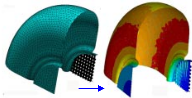
Figure 7: ANSYS FEA mesh and Heat flux results
