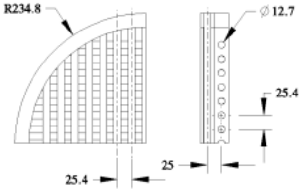
Figure 2: Layout of baseline grid window _ symmetry.
