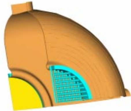
Figure 1: _ symmetry cutaway of 201MHz RF Cavity with closed irises using a beryllium window and a grid window.
