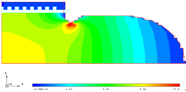
Figure 6: E_z field for case 2 - 15 x 15 array, grids touching. Excellent attenuation of fields past grid, excellent field quality near grids in cavity.
