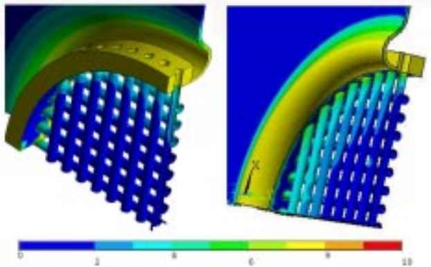
Figure 9: Temperature profile of grid using ANSYS.
