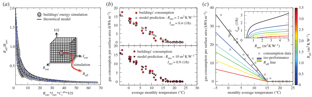
Figure 3. Estimation of buildings' gas consumption in dimensionless space via the response surface methodology. (a) Construction of the surrogate model in dimensionless form. Considering a dense full factorial grid in (I_{env}, R_{env}, V/S) space (as denoted in the inset), R_{eff} can be calculated at each point via building energy simulation using Energyplus. For a building with a given W_{typ} and N_c , the dimensional analysis yields that there exist only three dimensionless quantities relating R_{eff} to the rest of the influential parameters, I_{env} , R_{env} , V/S , C_v^{air} (volume heat capacity of air) and \eta_H , which are: \pi_1 = R_{eff}/R_{env} , \pi_2 = I_{env} \times R_{env} \times C_v^{air} V/S and \pi_3 = \eta_H . A surrogate model of the form \pi_1 = 1/\pi_3(C_1 + C_2 \times \pi_2) , as shown by the blue line, is fitted to the simulation results. Having the surrogate model at hand, we can estimate the performance of buildings without actually running the computationally expensive simulations. (b) Identification of buildings' thermal properties from monthly gas consumption data using the surrogate model. The solution of inverse problems to identify the buildings' characteristics such as I_{env} and R_{env} is non-unique. For instance, the surrogate model predicts the same R_{eff} value at two alternative cases of (I_{env} = 0.4 (1/h), R_{env} = 2 \text{ m}^2 \text{ K W}^{-1}) and (I_{env} = 0.9 (1/h), R_{env} = 10 \text{ m}^2 \text{ K W}^{-1}) located on an iso-performance line. (c) Estimation of retrofit gas savings at the building level. Given the monthly gas consumption of the building, R_{eff} is estimated by fitting a line denoted in black. The associated R_{eff} attributes to the black iso-performance line in the inset in (R_{env}, I_{env}) space. By performing retrofit, the R_{eff} of the building increases. The colours of iso-performance lines match the colours for gas consumption per surface area in the main graph. Therefore, the higher increase in R_{eff} directly translates to higher gas savings upon retrofit.
