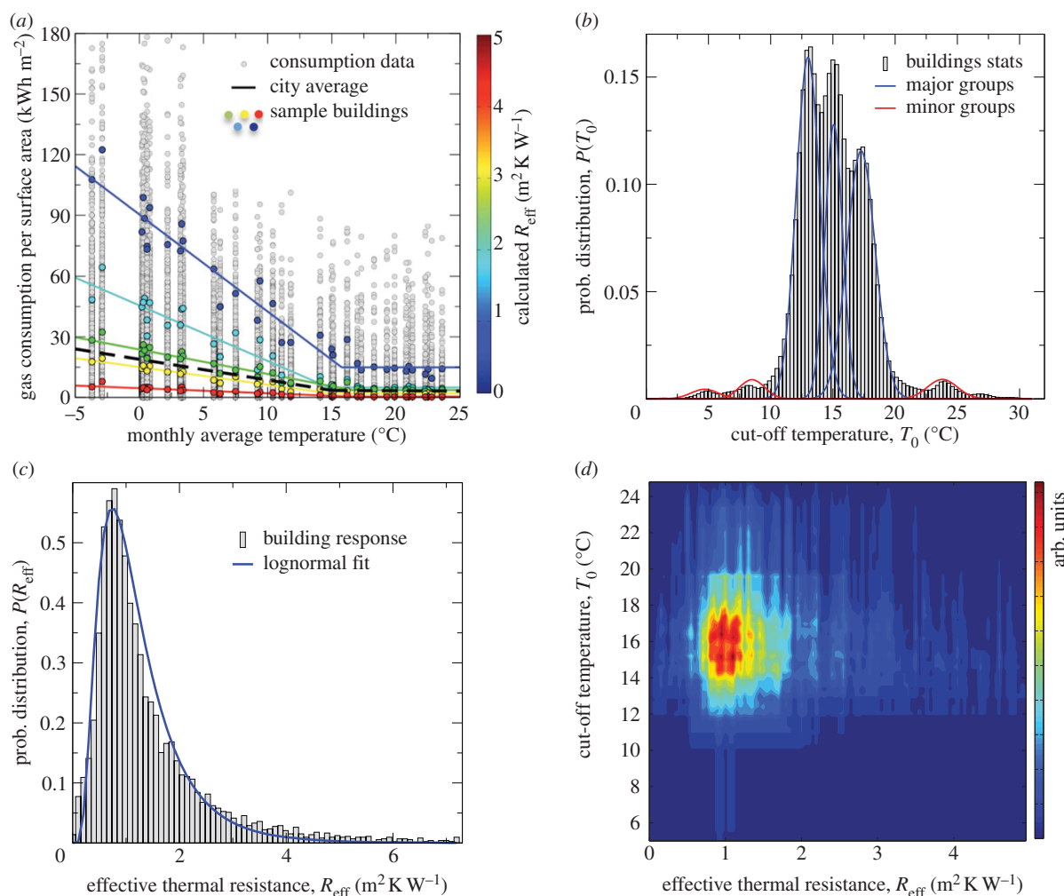
Figure 1. Data assimilation and analysis by integration of various data sources including buildings' footprints, weather data and gas consumption bills. (a) Gas consumption per surface area as a function of monthly average temperature for more than 6200 buildings in a period of 2007–2009 in Cambridge, MA, USA. The average city consumption per surface area is shown by the dashed black line. Five sample buildings are highlighted based on their effective thermal resistance defined in equation (2.1). The gas consumption of the buildings exhibits a piecewise linear trend with gas consumption increasing below a certain temperature threshold. (b) Distribution of the cut-off temperature indicating the variability of consumers' perception of and resistance to cold weather. (c) Distribution of effective thermal resistance for all the buildings. The Gaussian mixture analysis identifies the three major populations of the consumers that turn on their heating system at 17°C, 15°C and 13°C on average. The distribution of effective normal resistance follows a lognormal distribution, with an average value of 1 m 2 K W -1 . (d) The joint probability distribution function of the T 0 and R eff . The absence of correlation suggests that the energy consumption of buildings and the consumers' behaviour are not correlated.
