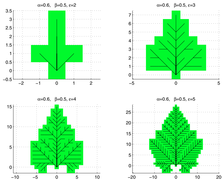
FIGURE 1. \alpha = 0.6, \beta = 0.5 .
