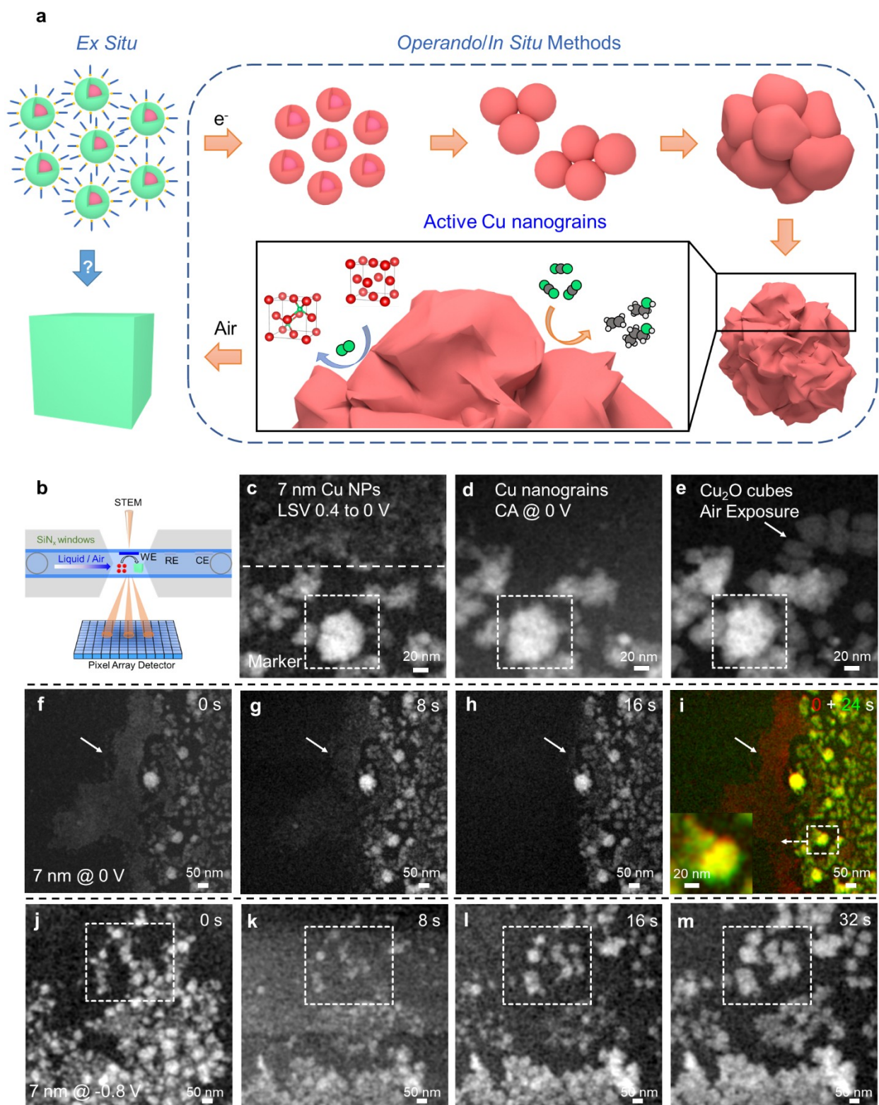
Figure 1. Operando correlative studies of dynamic electroreduction/reoxidation life cycle of Cu nanocatalysts. (a) Conventional ex situ methods are limited to the study of nanocatalysts before/after CO 2 RR. In contrast, operando/in situ methods used in this study, including EC-
