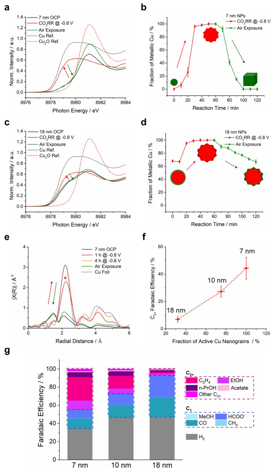
Figure 4. Operando HERFD XAS studies of the valence state and coordination environment of Cu nanocatalysts during their electroreduction/reoxidation life cycle. (a) Operando HERFD XANES spectra of pristine 7 nm NPs, metallic Cu formed at -0.8 V under CO 2 RR conditions and Cu 2 O cubes formed upon post-electrolysis air exposure, along with the standard
