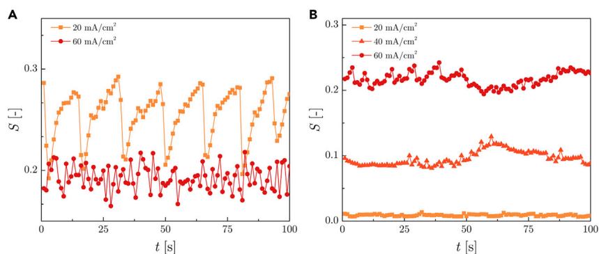
Figure 4. Evolution in Local Gas Saturations
