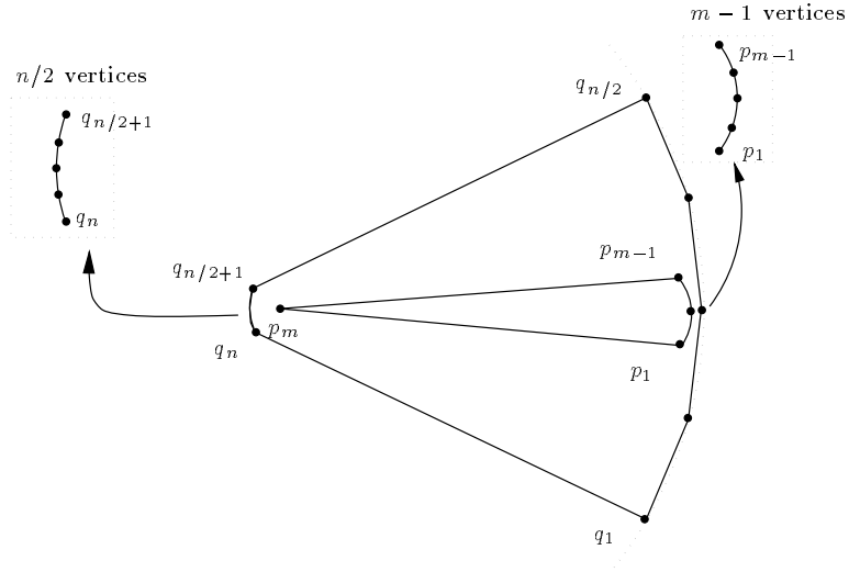
Figure 4: Polygons P and Q for which there exist \Omega(mn^2) similar placements of P in Q with four vertex-edge incidences per placement
