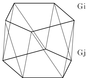
Figure 2: Convex hull of parallel polygons
