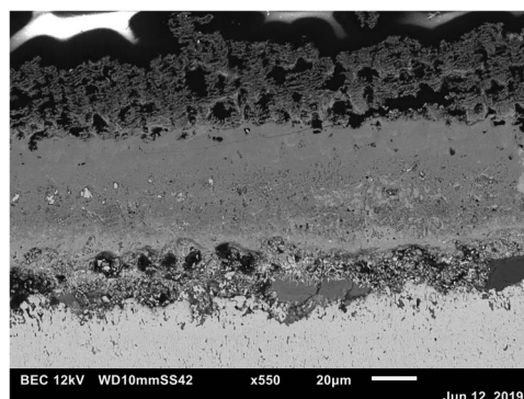
Figure 6. Backscattered electron image of cross-sectioned Alloy 718 sample exposed at 750^\circ\text{C} in \text{Na}_2\text{SO}_4\text{-NaCl} .
