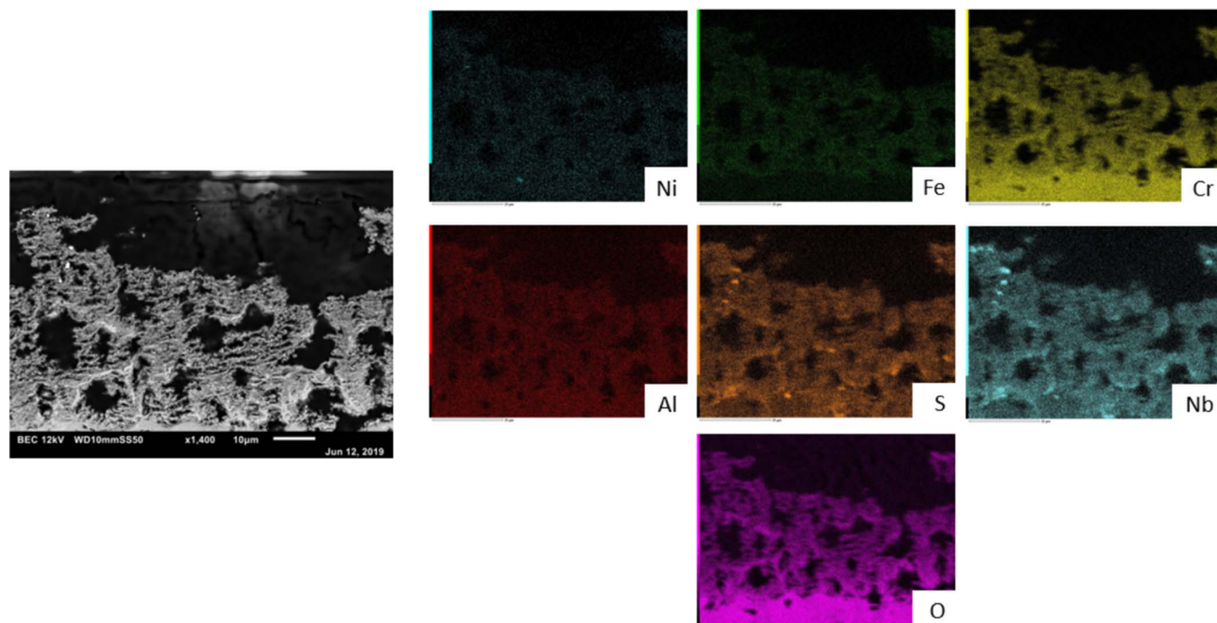
Figure 7. Higher magnification backscattered electron image and corresponding EDS elemental maps of the outer (porous) layer shown in Figure 6.
