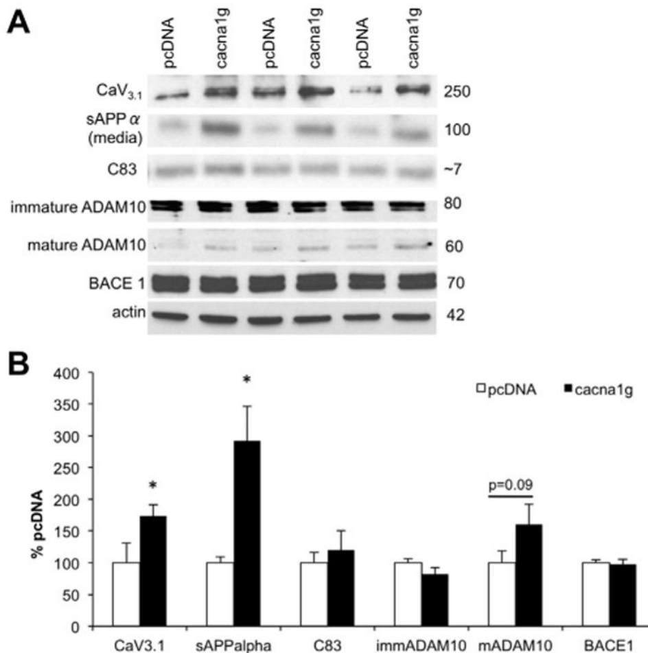
Fig. 6. Overexpression of cacna1g produces complementary effects to NNC-55-0396 in HEK69 cells. We achieved a 74% overexpression of the CaV 3.1 T-type channel in HEK269 cells, which coincided with a significant increase in secreted APP \alpha and a trend toward an increase in mature ADAM10 levels, while BACE1 levels remained unchanged (A, quantified in [B]). * p < 0.05 .
