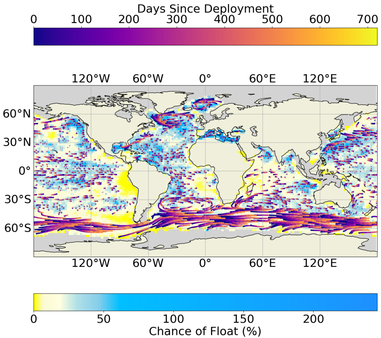
FIG. 6. Two year prediction of array density of global Core Argo array. Argo array distribution is based on the May, 2021 snapshot (Argo 2021) using the transition matrix (Chamberlain et al. 2023) (Eq. 23). Colored lines represent time of mean transition ( t in Eq. 24). Grid cell shading represents estimated array density. Gray shading represents areas outside domain of the transition matrix; beige shading represents land.
