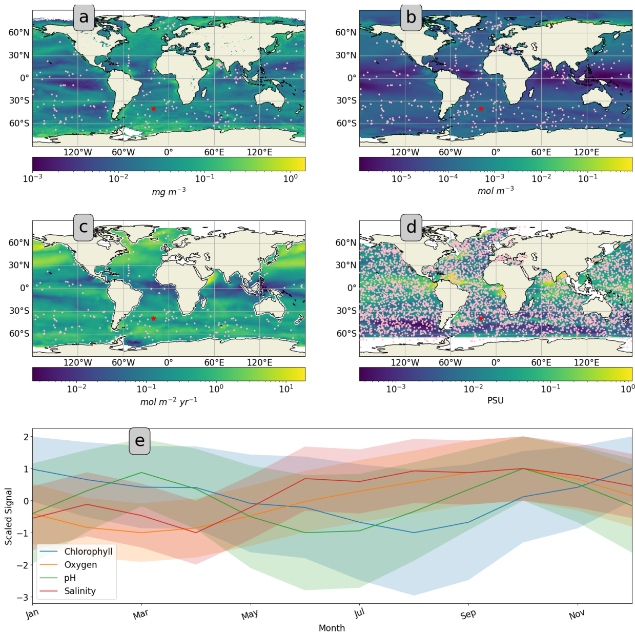
FIG. 3. (a-d) Maps of standard deviation of a) chlorophyll (NASA 2022), b) oxygen (CM4), c) \text{CO}_2 flux (Landschützer et al. 2016), d) salinity (Roemmich and Gilson 2009). Pink dots represent deployed floats with a sensor equipped to measure a) chlorophyll, b) oxygen, c) pH, d) salinity. Colored shading represents the standard deviation of the variable. Beige shading is land. e) Monthly mean and anomaly from annual mean normalized by standard deviation from CM4 for chlorophyll (blue line), oxygen (orange line), pH (green line), and salinity (red line) at 40°S, 20°W (denoted by red star on all maps).
