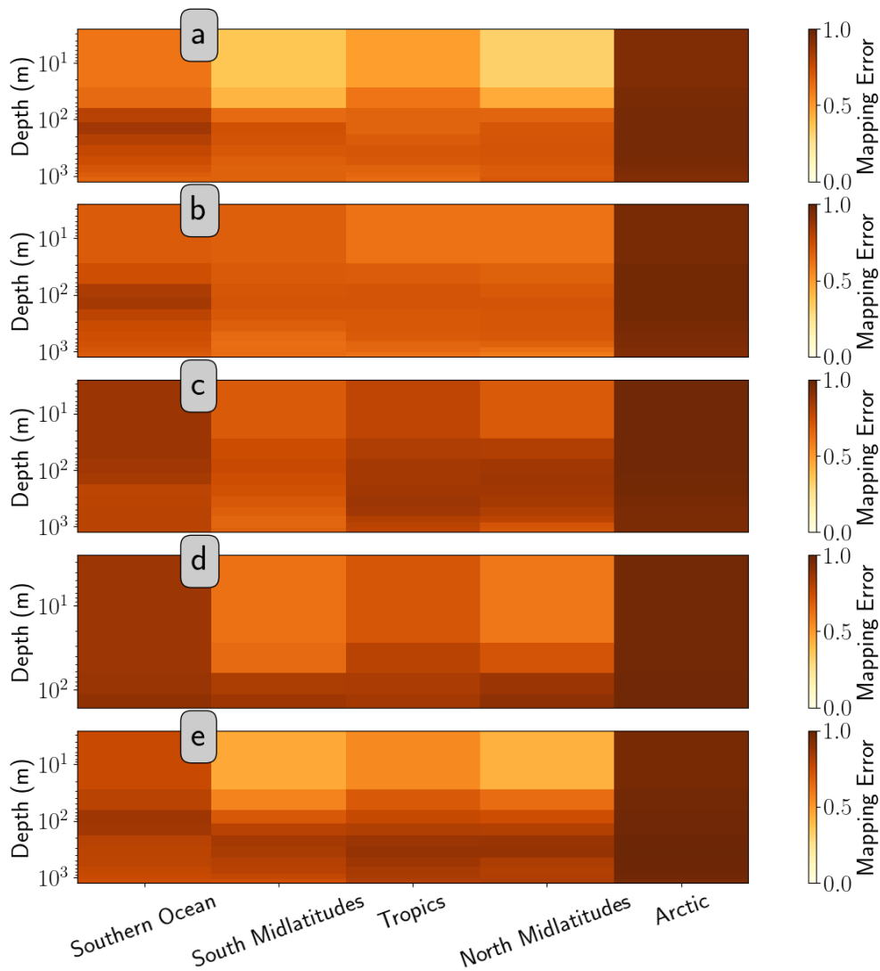
FIG. 9. Zonal average formal mapping error ( E^{map} ) of existing Argo core and BGC float array at all depths of a) temperature, b) salinity, c) pH, d) chlorophyll, and e) oxygen. (Zones are defined by Southern Ocean: south of 60^\circ\text{S} , South Midlatitudes: 60^\circ\text{S} - 20^\circ\text{S} , Tropics: 20^\circ\text{S} - 20^\circ\text{N} , North Midlatitudes: 20^\circ\text{N} - 60^\circ\text{N} , Arctic: north of 60^\circ\text{N} .)
