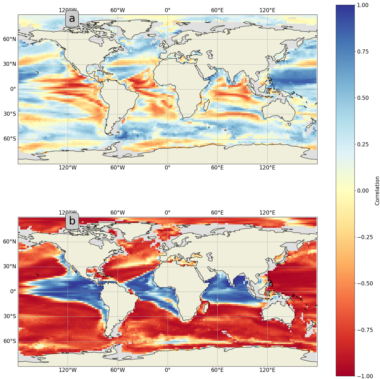
FIG. 2. Global Climate Model (CM4) (Held et al. 2019; Adcroft et al. 2019; Dunne et al. 2020) correlation maps of a) chlorophyll and oxygen and b) temperature and oxygen at a depth of 100 m. Colored shading represents strength of correlation. Beige shading represents land. Gray areas are too shallow to be calculated in simulations.
