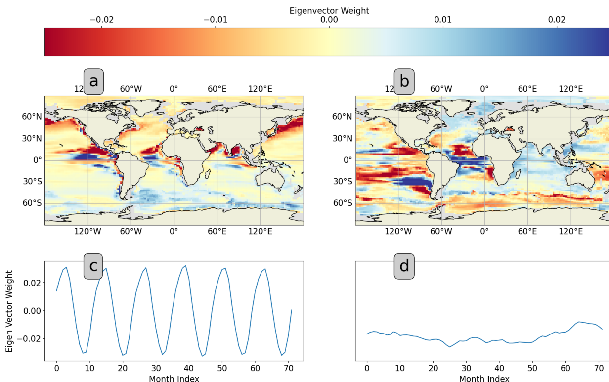
FIG. 5. (a and b) CM4 maps of eigenvectors of spatial pH covariance for a) the gravest mode at 100 m depth and b) the gravest mode at 1000 m depth. Colored shading represents the covariance weighting, beige shading indicates land. (c and d) 72 month subsets of eigenvectors of temporal pH covariance for c) the gravest mode at 100 m depth and d) the gravest mode at 1000 m depth. Gravest mode at 100 m depth explains 15.5% of the variance, gravest mode at 1000 m depth explains 6.9 % of the variance.
