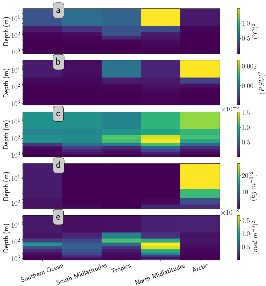
FIG. 10. Zonal average analysis error covariance \mathbf{P}^a of existing Argo core and BGC float array at all depths, of a) temperature, b) salinity, c) pH, d) chlorophyll, and e) oxygen. (Zones are defined by Southern Ocean: south of 60°S, South Midlatitudes: 60°S - 20°S, Tropics: 20°S - 20°N, North Midlatitudes: 20°N - 60°N, Arctic: north of 60°N.)
