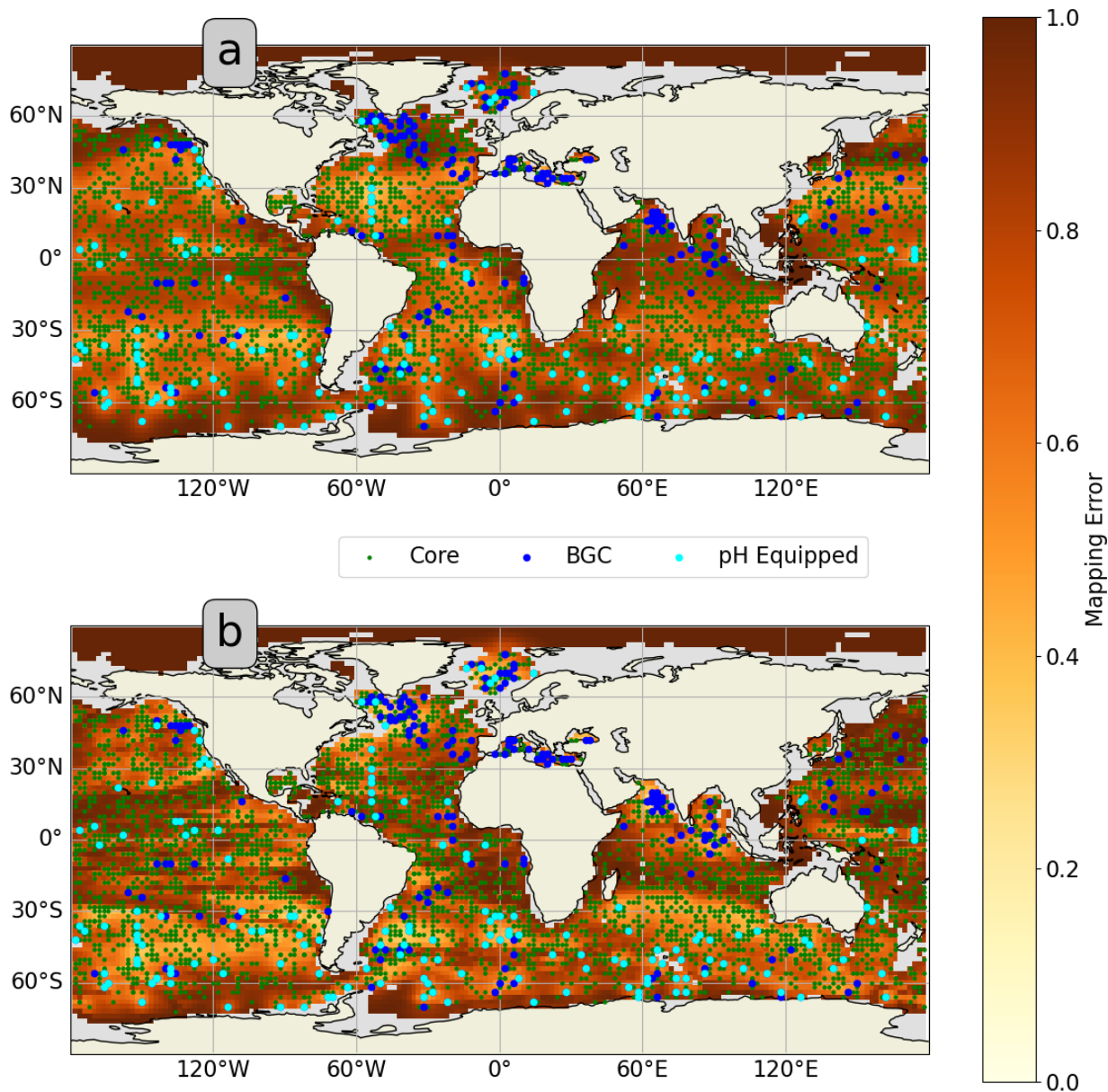
FIG. 8. Scaled pH formal mapping error ( E^{map} ) of existing core and BGC Argo float array taken from May, 2021 snapshot at a) the surface and b) 1000 meters. Colored shading represents amount of unconstrained variance. Beige shading represents land. Gray areas are too shallow. Green dots represent core Argo floats. Blue dots represent BGC Argo floats without pH sensors. Cyan dots represent BGC floats equipped with pH sensors.
