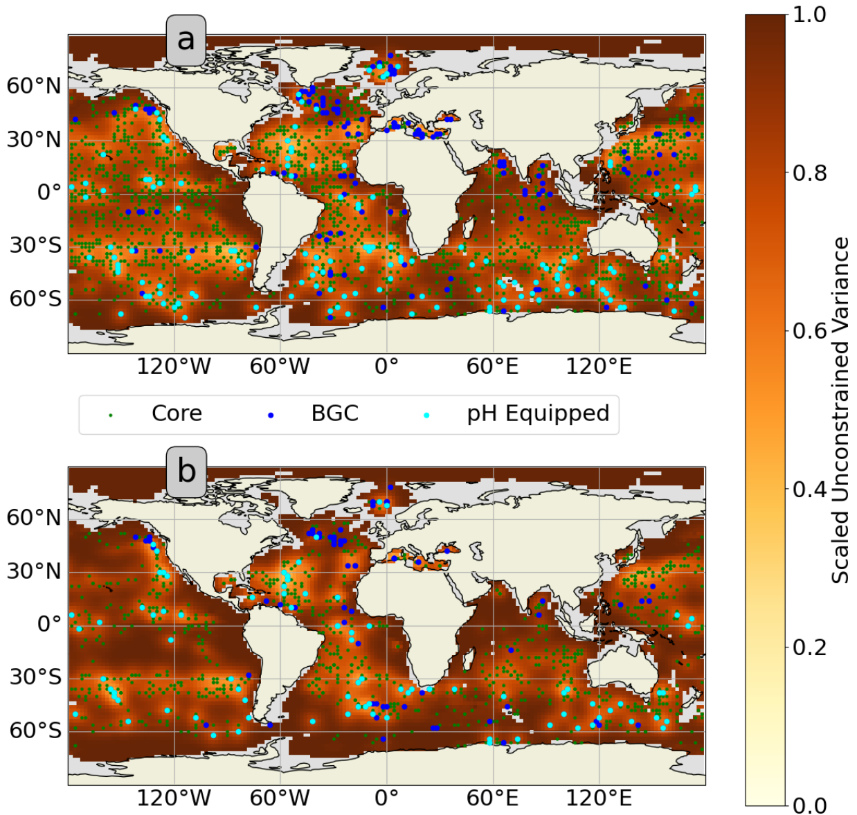
FIG. 12. Scaled surface pH formal mapping error ( E^{map} ) of the Argo float array of May, 2021, projected at a) one and b) two years into the future assuming floats are not replenished. Colored shading represents amount of E^{map} . Beige shading represents land. Gray areas are too shallow to be calculated in simulations. Green dots represent location of existing core Argo floats. Blue dots represent location of existing BGC Argo floats. Cyan dots represent floats equipped with pH sensors.
