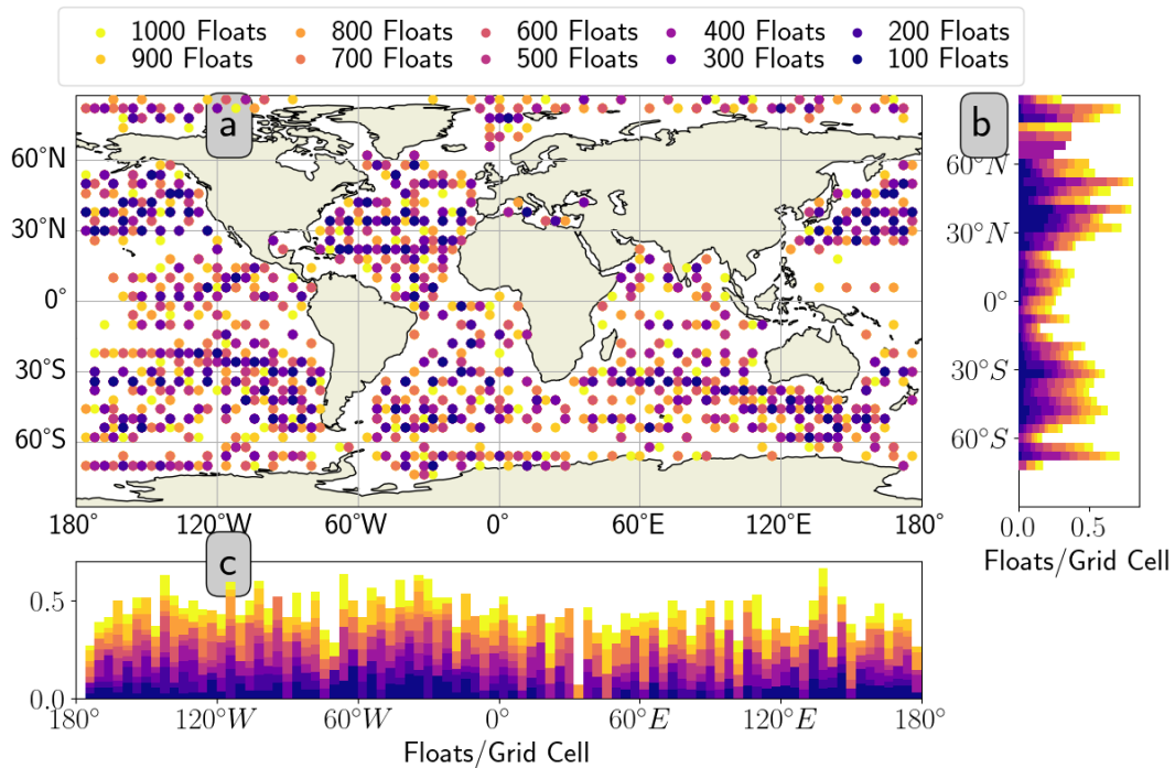
FIG. 15. a) Map of the optimal distribution of 1000 BGC Argo floats with a grid spacing of approximately 6° in latitude and longitude. Dots represent ideal BGC Argo float locations for observing the BGC anomalies from the mean. State vector used for calculation is based on 4 depth levels (15 m, 87.5 m, 550 m, and 950 m) of CM4 BGC output at a grid spacing of 4° in latitude and longitude. Beige shading indicates land. b) Histogram of zonally binned optimal array. c) Histogram of meridionally binned optimal array. Both histograms binned in increments of 6° latitude and longitude respectively. Colored shading indicates when in the sequential calculation floats were deployed (i.e. purple indicates locations identified first, yellow indicates locations identified last). Float locations identified earlier are relatively more important in this optimal configuration by construction.
