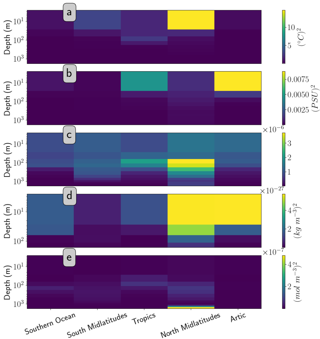
FIG. A4. Zonal average of total variance (diagonal of \mathbf{P} ) for all variables and depths.
