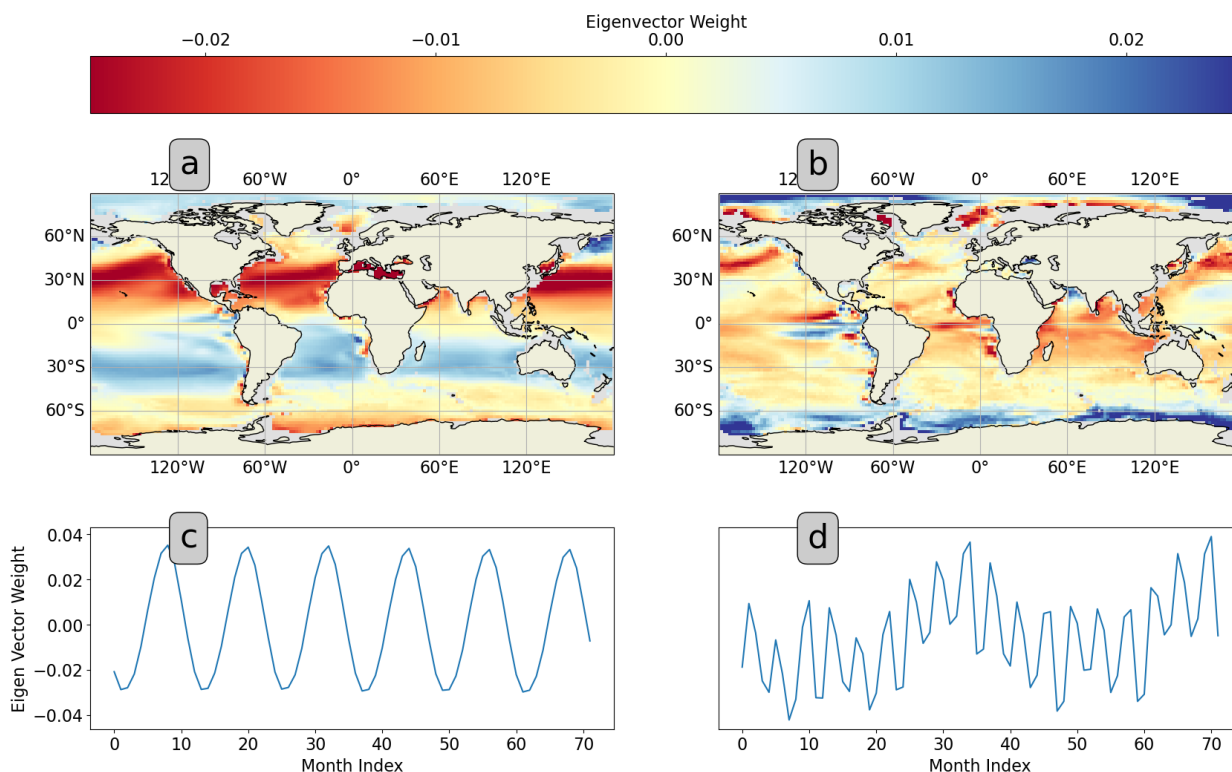
FIG. 4. (a and b) CM4 maps of eigenvectors of spatial surface pH covariance for a) the gravest mode and b) the 7 th eigenmode. Colored shading represents the covariance weighting, beige shading indicates land. (c and d) 72 month subsets of eigenvectors of temporal surface pH covariance for c) the gravest mode and d) the 7 th eigenmode. Gravest mode explains 14.0% of the variance, 7 th eigenmode explains 0.8 % of the variance. The 1st and 7th eigenmodes are shown as an example to explain the scaling argument of section 3 c.
