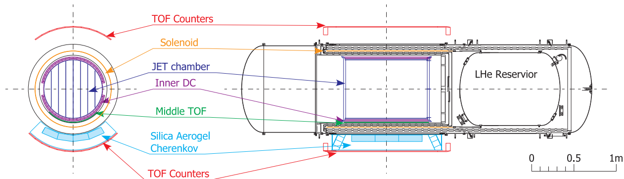
Figure 1: The BESS-Polar II experiment consists of inner drift chambers and a jet-type drift tracking chamber, surrounded by a solenoid magnet, aerogel Cherenkov counter, and time-of-flight system.
