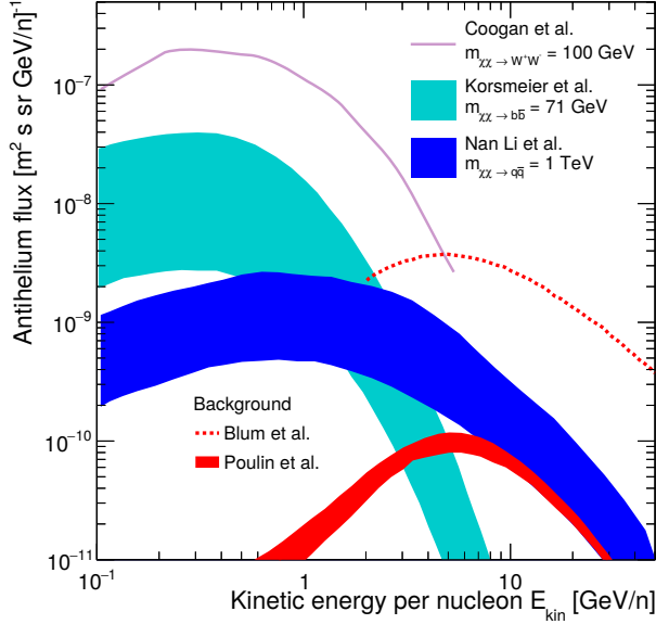
Figure 6: Antihelium-3 flux predictions from different DM model and astrophysical background calculations [38, 41, 47, 50, 51]. The error bands illustrate uncertainties in the coalescence momentum, but also include propagation uncertainties.
