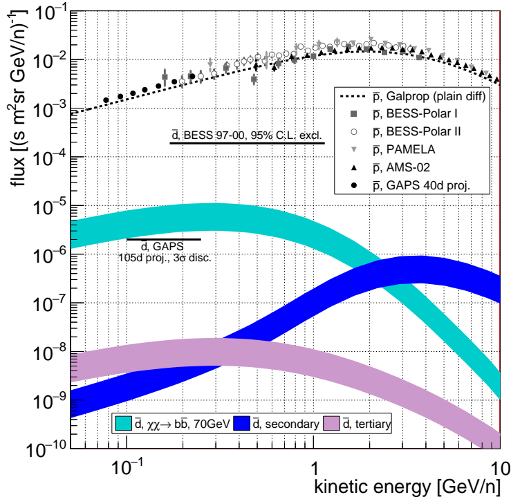
Figure 7: Antiproton flux data from AMS-02 [8], BESS-Polar I/II [4, 103], and PAMELA [6], as well as projections for the GAPS [89] antiproton flux measurements after 40 days, in comparison with the GALPROP plain diffusion prediction [104]. Also shown are the predicted antideuteron flux corresponding to DM parameters indicated by AMS-02 antiproton signal, interpreted as annihilation into purely b\bar{b} [38, 96]), as well as the predicted secondary and tertiary astrophysical antideuteron flux. The anticipated sensitivity of GAPS [55] for a 3\sigma discovery and the BESS 97–00 95% C.L. exclusion limits are indicated [53]. Solar modulation is treated in the force-field approximation with a potential of 500 MV. All antideuteron fluxes are derived in the analytic coalescence model with a coalescence momentum of 160 GeV [97] for the lower edge of the band and with a higher coalescence momentum of 248 GeV [98] for the upper edge of the band.
