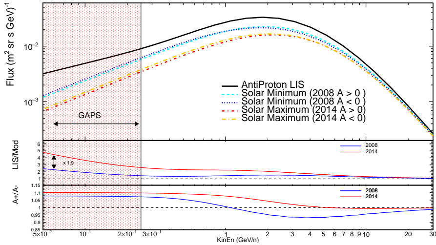
Figure 11: Top panel: Antiproton flux for solar minimum and maximum from a 3D numerical model for cosmic-ray propagation through the Heliosphere. The solar minimum and solar maximum spectra has been evaluated for positive and negative polarity of the HMF ( A > 0 and A < 0 ) to show the effect of the charge sign solar modulation. Middle panel: Ratio between the LIS and the modulated spectra for the period of maximum and minimum solar activity ( A < 0 ). Bottom panel: Ratio between the modulated spectra for opposite polarity of the HMF for the period of minimum and maximum solar activity.
