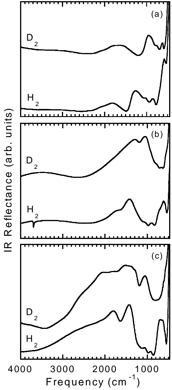
Figure 3. Internal reflectance infrared spectra of (a) 400 nm Mn-Mg, (b) 385 nm Fe-Mg, (c) 250 nm Co-Mg films on ZnSe substrates following loading in H 2 and D 2 .
