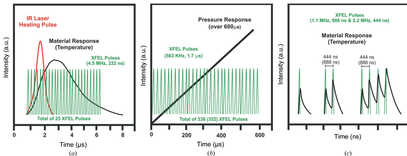
Figure 1 Schematic views of the expected timing for (a) infrared laser heated DAC and (b) dDAC experiments in the DAC setup for the HED instrument at the European XFEL. In the case of the dDAC experiment the limiting factor will be the fact that the AGIPD will only be able to collect 352 images. (c) Schematic of the single X-ray exposures and pump-probe approaches used during the 1st UCAC experiment. Consecutive diffraction patterns from one pulse train are accumulated in one image from the VAREX XRD 4343CT. The green pulses represent the X-ray pulses of 17.8 keV delivered within one train, while the black lines indicate the material response, such as an increase in temperature.
