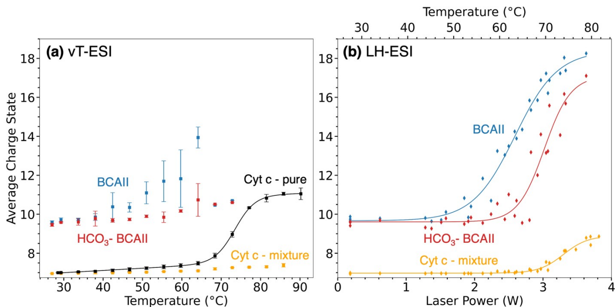
Figure 2. Average charge state of apo- and bicarbonate-bound BCAII (blue/red) and cyt c (orange/black) obtained by (a) vT-ESI or (b) LH-ESI from a solution containing 7:3 BCAII: cyt c in 50 mM ammonium acetate. LH-ESI data are shown as a function of laser power (bottom axis) and recalibrated temperature (top axis). BCAII signal above \sim 68 °C in (a) was observed in only one replicate. Data in black were obtained from a solution containing 10 \mu\text{M} cyt c in 20 mM ammonium acetate. There are no BCAII ions above \sim 72 °C in vT-ESI experiments due to irreversible aggregation, preventing the measurement of a full melting curve for this protein.
