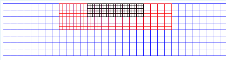
Appendix 1—figure 1. Schematic view of a nested finite difference grid for the agar region \Omega_2 .
