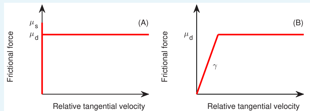
Appendix 1—figure 2. The standard (A) and modified (B) model for friction between two objects, as a function of tangential relative velocity between the two objects, where \mu_s and \mu_d are the static and dynamic friction constants, respectively.
