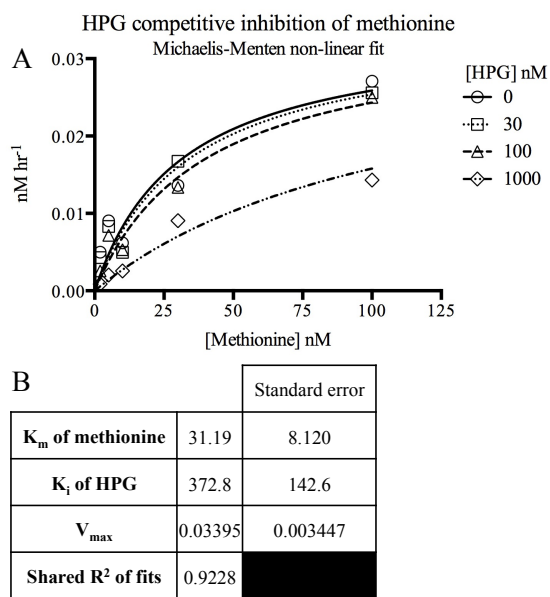
Figure 4.4. Michaelis-Menten enzyme kinetics chart displaying HPG competitive inhibition of methionine (A). Summary values of fitted values calculated from each dataset (B).
