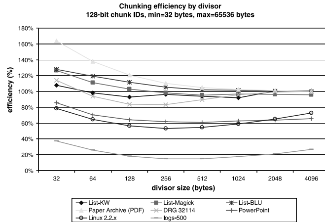
Fig. 9. Chunking efficiency by divisor size.
