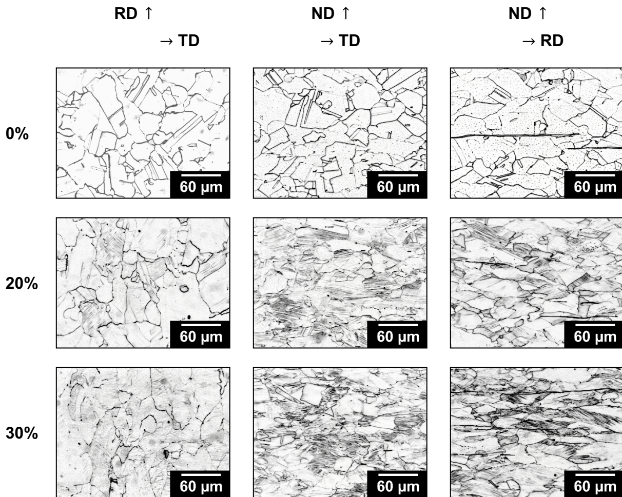
Figure 8: Etched micrographs showing deformation after rolling (elongating grains in RD) deformation twins (darkened areas within grains in 20% & 30% conditions), and ferrite stringers (black lines parallel to RD).
