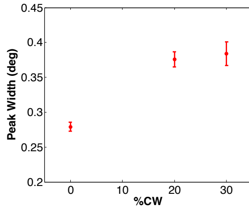
Figure 14: XRD peak width (FWHM) averaged over all nine samples per each CW condition. Error bars are one standard deviation
