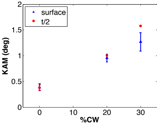
Figure 11: KAM as a function of CW condition for several scans. Results for both near-surface and bulk material are included.
