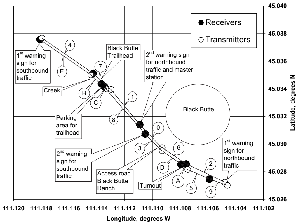
Figure 1. Schematic layout of the animal detection system and major road and landscape features at the study site (Source: STS). The numbers and letters represent the codes of the individual detection zones.
