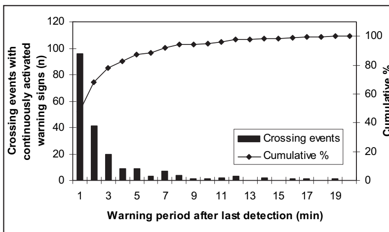
Figure 12. The number of crossing events with continuously activated warning signs (warning lights remain active during the entire crossing event) given a certain warning period after the last detection. The results are based on the crossing events between 27 January 2005 and 14 February 2005, 19 February 2005 and 21 February 2005, and 26 February 2005 and 5 March 2005. The line represents the cumulative percentage of all crossing events (see text).
