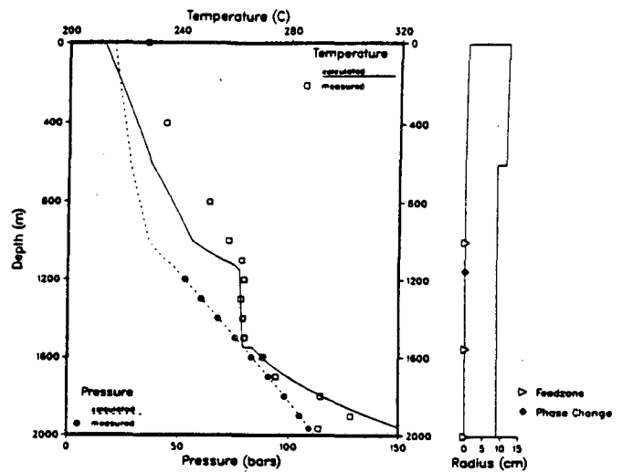
Nesjavellir, well NJ-7 Pressure and enthalpy during discharge 6-feb-1986
