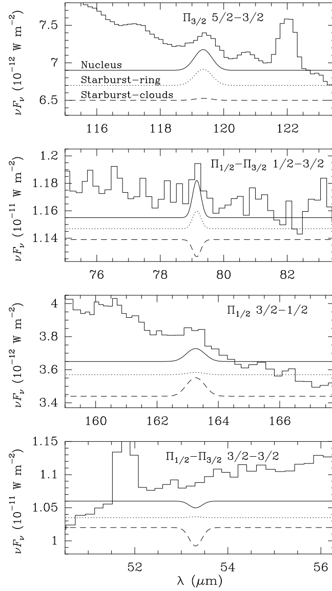
FIG. 6.— Comparison between the observed OH lines and model results. As indicated in the upper panel, the upper modeled spectrum (solid lines) corresponds to the model for the nucleus, the middle one (dotted lines) corresponds to the starburst modelled as a whole, and the lower one (dashed lines) corresponds to the starburst modelled as an ensemble of individual clouds (see text for details).
