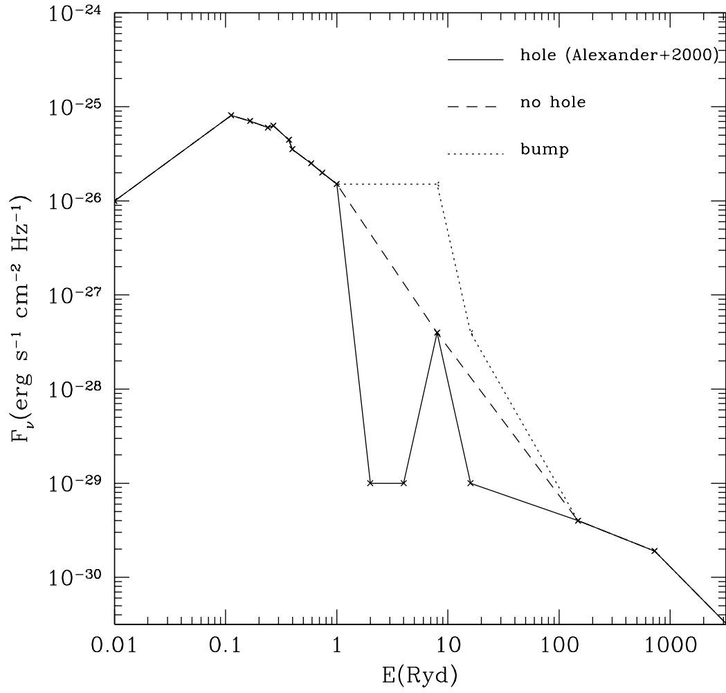
FIG. 1.— The AGN ionizing continua used as input for the photoionization models of NGC 1068. The three continua differ in the frequency region between 1 > E_{Ryd} > 100 , while outside this region the Pier et al. (1994) spectrum was adopted. The solid line shows the continuum derived from Alexander et al. (2000); the dashed line shows a simple power law interpolation; the dotted line shows the presence of the predicted "big blue bump".
