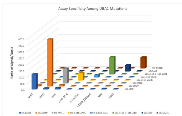
Fig. 3. Signal/noise ratio (SNR) of all mutant assay in the presence of each mutant synthetic DNA at 5%.
