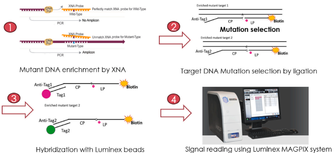
Fig. 2. Overview of the QClamp Plex assay. The four assay steps are: (1) XNA clamping PCR for mutant target enrichment; (2) allele specific ligation to label mutant target with biotin and Tag sequences; (3) capture of the specific mutant targets to their corresponding beads through Tag-antiTag hybridization; and (4) Hybridization with SAPE and analysis of beads intensity signal with Luminex system.
