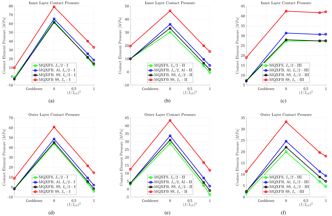
Fig. 7. Evolution of the contact pressure during magnet loading, cooldown and powering at nominal and ultimate current, computed with numerical models on the locations shown in Fig. 6. The stress on the rods is given in Table II. (a): IL, I. (b): IL, II. (c): IL, III. (d): OL, I. (e): OL, II. (f): OL, III.
