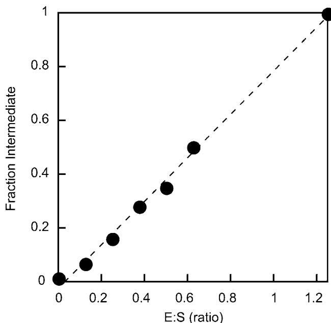
Figure 9. Covalent Enzyme-Intermediate Formation Is Stoichiometric with APS Reductase
