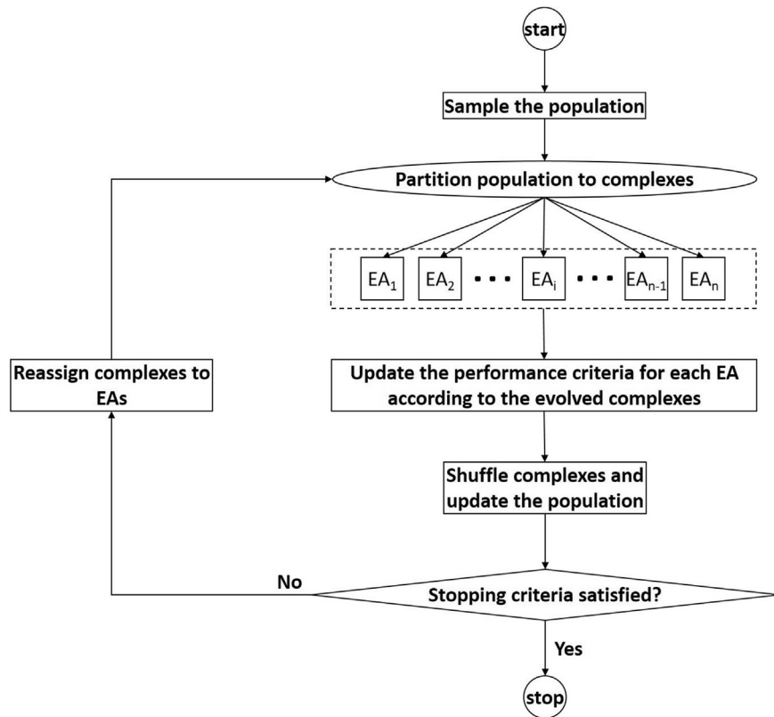
Fig. 1. The SC-SAHEL framework flowchart.
