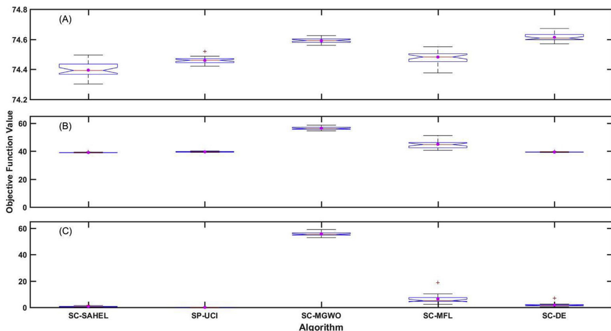
Fig. 8. Boxplots of objective function values for successful runs among 30 independent runs, for dry (A), below-normal (B) and wet period (C). The mean of objective functions values is shown with pink marker. (For interpretation of the references to colour in this figure legend, the reader is referred to the Web version of this article.)
