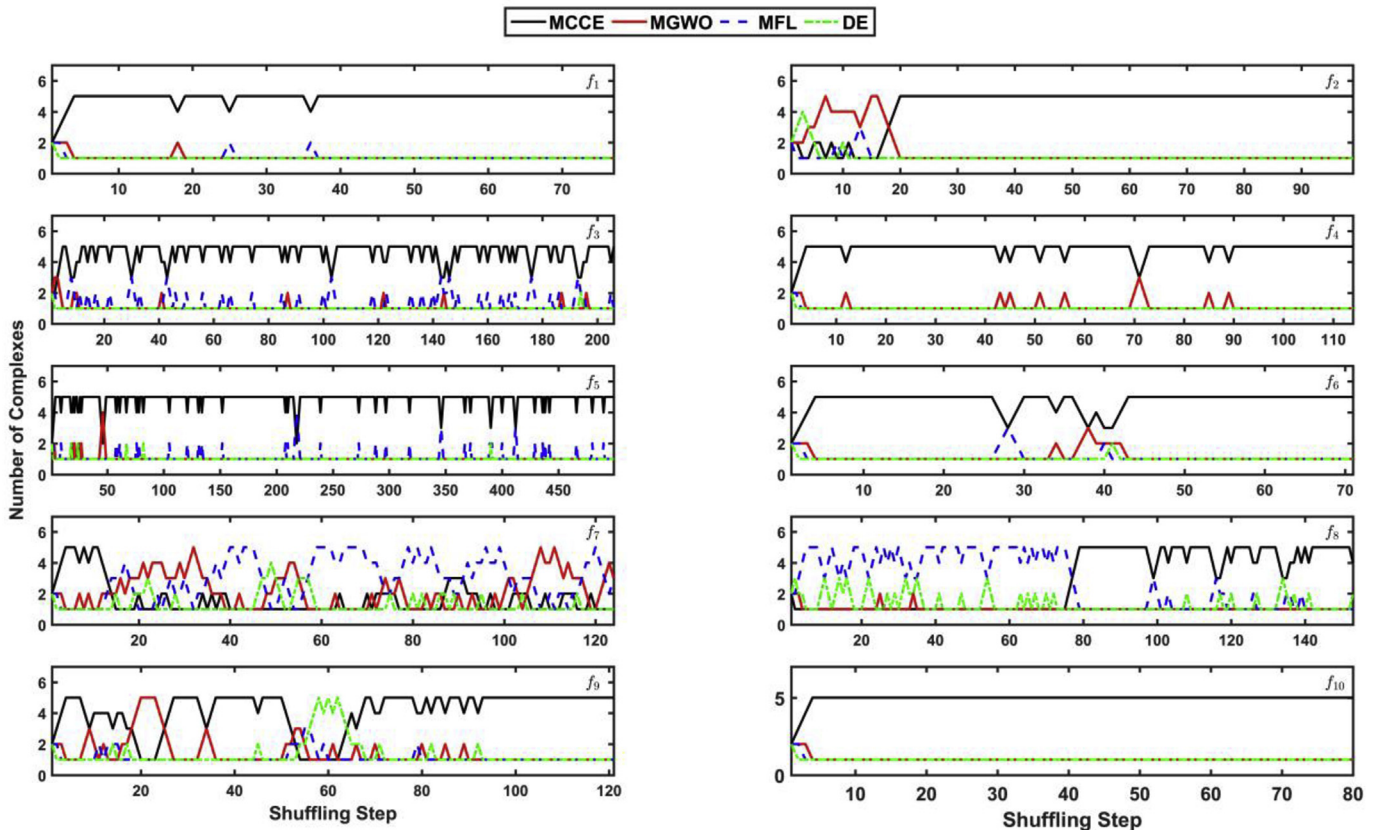
Fig. 5. Number of complexes assigned to EAs during the entire optimization process for test functions f_1 - f_{10} .
