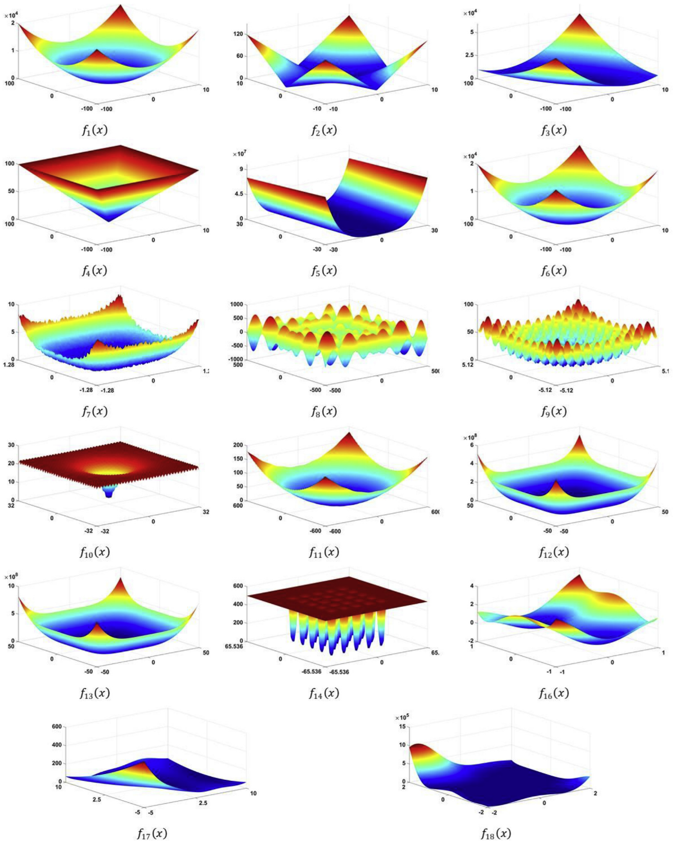
Fig. 2. Classic test functions in 2-dimension form.
