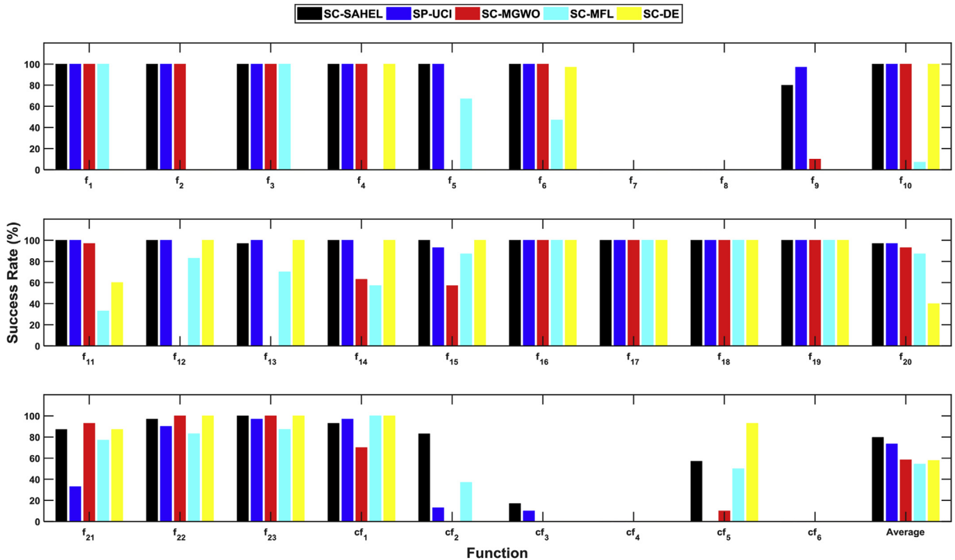
Fig. 4. The success rate of the SC-SAHEL algorithm using multi-method and single-method search mechanism for 30 independent runs for 29 test functions.
