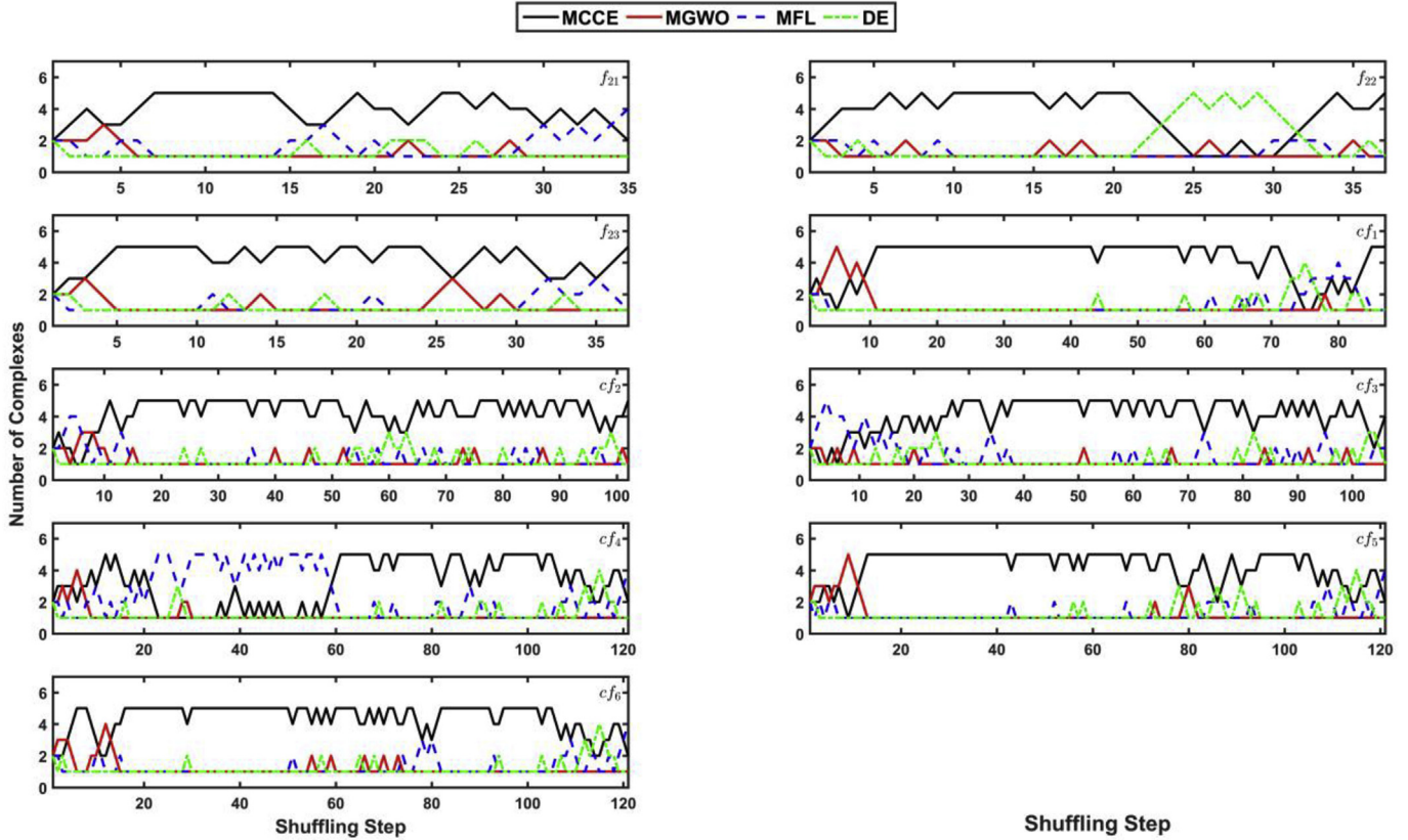
Fig. 7. Number of complexes assigned to EAs during the entire optimization process for test functions f_{21} - f_{23} and cf_1 - cf_6 .
