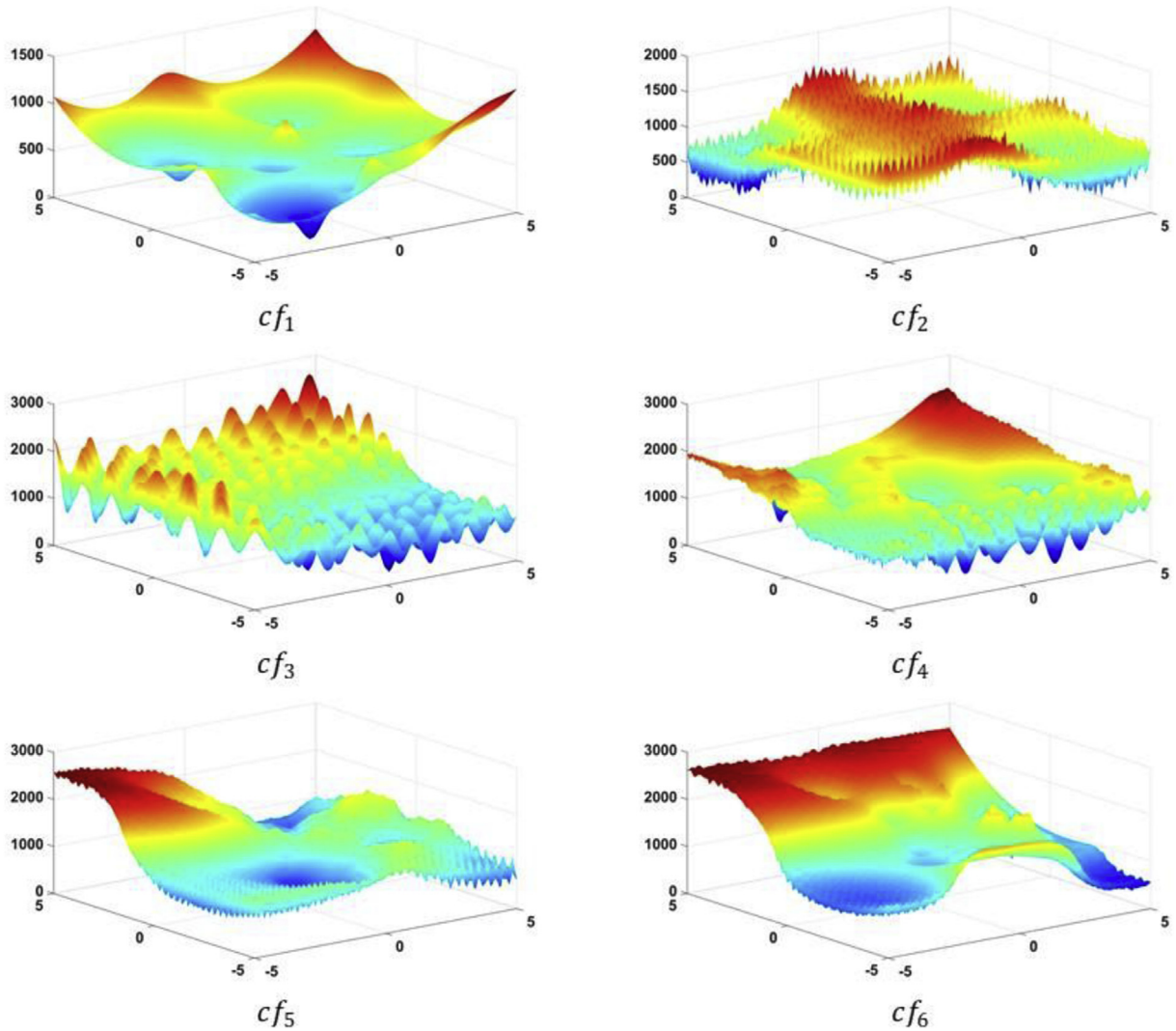
Fig. 3. Composite test functions in 2-dimension form.
