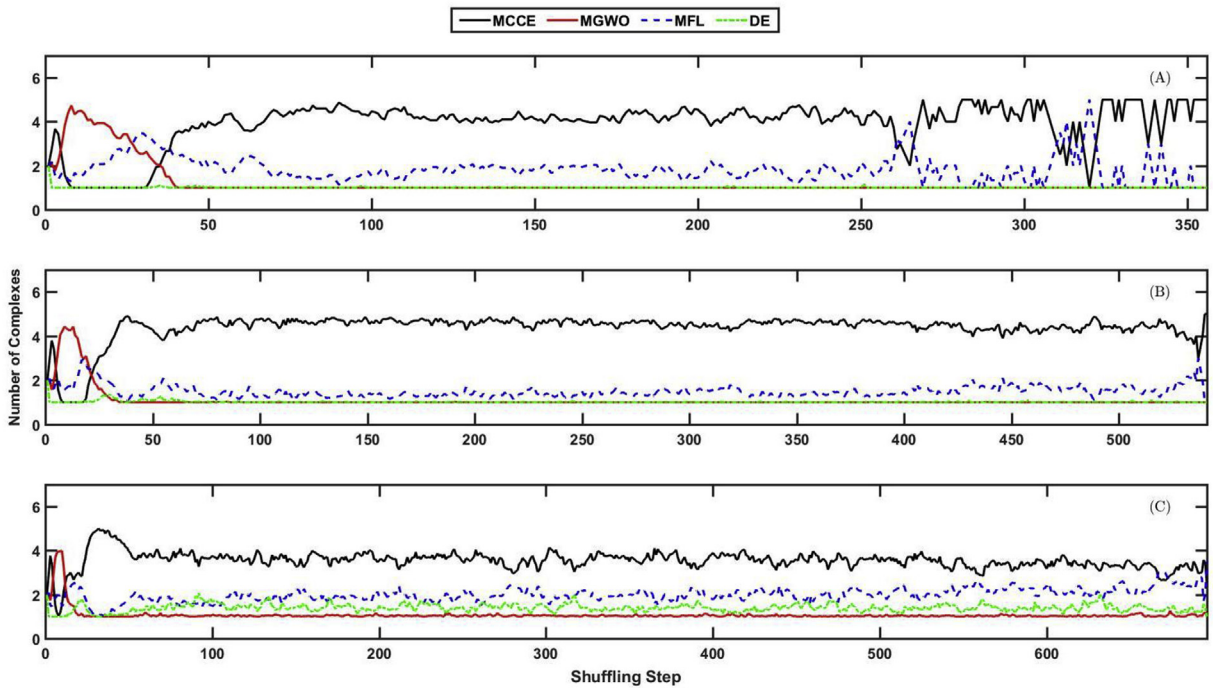
Fig. 10. The average number of complexes assigned to each EA at each shuffling step for 30 independent runs for dry (A), below-normal (B), and wet (C) period.
