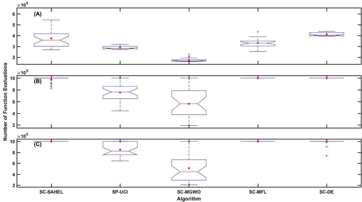
Fig. 9. Boxplots of number of function evaluations for successful runs among 30 independent runs for dry (A), below-normal (B) and wet period (C). The mean number of function evaluation is shown with pink marker. (For interpretation of the references to colour in this figure legend, the reader is referred to the Web version of this article.)
