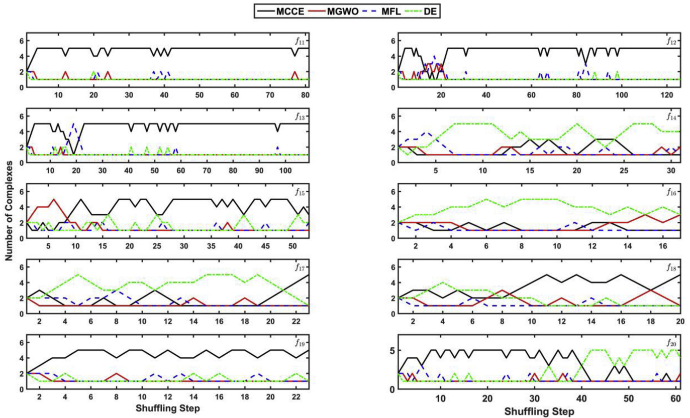
Fig. 6. Number of complexes assigned to EAs during the entire optimization process for test functions f_{11} – f_{20} .
