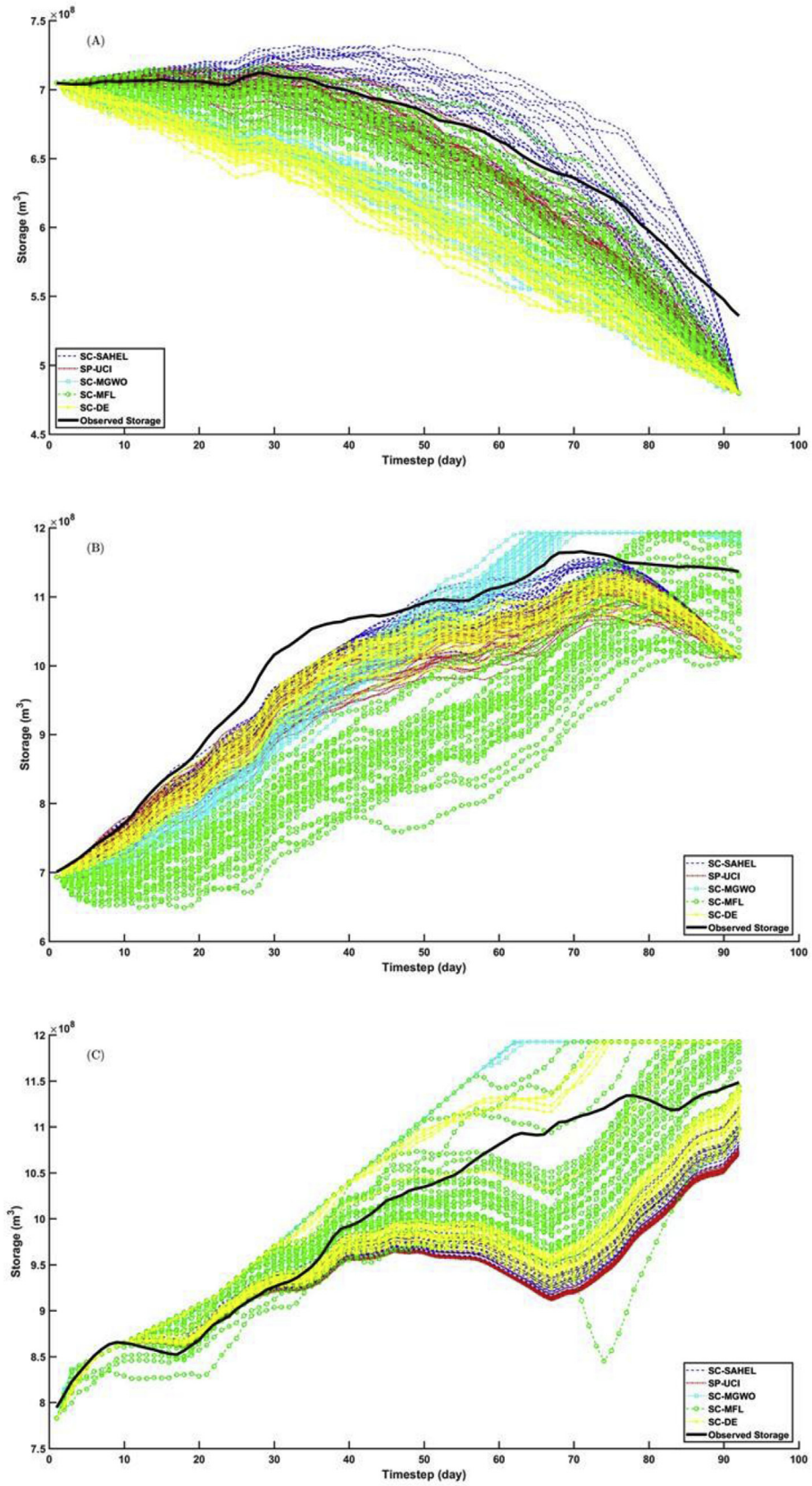
Fig. 11. Simulated storage for dry (A), below-normal (B), and wet (C) period.
