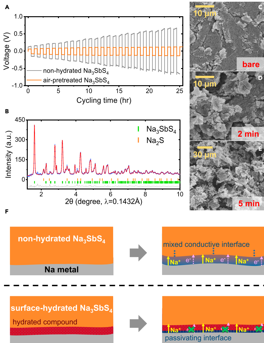
Figure 1. Enhancement of Na/Na 3 SbS 4 Interfacial Stability via Surface Hydration of Solid-State Electrolyte
