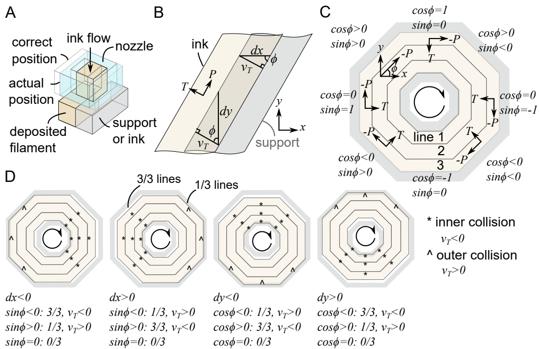
Figure 7.S9: A) The nozzle origin is calibrated too far to the right, resulting in collisions between ink and existing support or ink. B) Collisions induce a transverse flow v_T . C, D) The number of passes around the polygon which feature collisions with existing features depends on the printing direction \phi .
