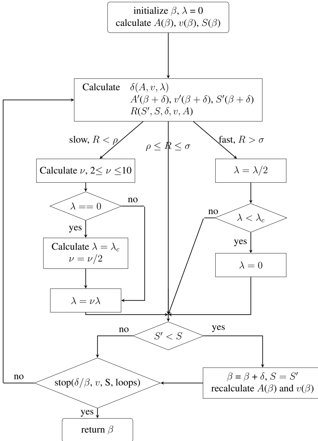
Figure 3.6: The Levenberg-Marquardt-Fletcher algorithm. Fletcher suggests \rho = 0.25 and \sigma = 0.75 . [157]
