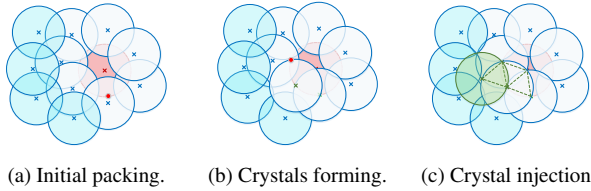
(a) Initial packing. (b) Crystals forming. (c) Crystal injection. Figure 4: Crystal growth injection of a uniform packing. Disks move to form “crystals” of equilateral triangles. Once a void is created, a new disk is inserted there.
