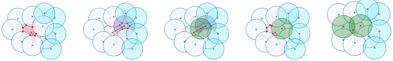
(a) A disk with center p is selected (randomly). Identify its unique void/corners. (b) Pick a neighboring disk center q_1 , and find the corners of its void. (c) Move q_1 along segment pq_1 as far as possible without uncovering q_1 's unique void. (d) If any void remains, find a neighbor q_2 at a different corner, and move it as in (c). (e) Repeat (c)–(d) until p 's whole void is covered and we can eject p .
