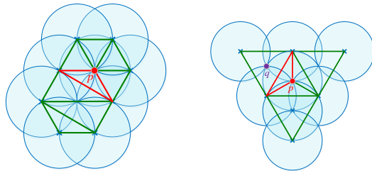
(a) Injection needed at circum-center of obtuse triangle. Ejection creates new obtuse angle. (b) Ejection is needed because p is trivalent. Injecting q would create new obtuse angles.
