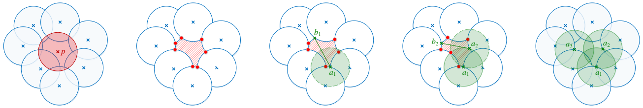
(a) A disk with center p is selected (randomly) as the candidate region for injection. (b) Disk p is removed, temporarily spoiling coverage. Void corners identified. (c) A new disk is injected at either of the two corners that are farthest apart ( a_1, b_1 ). (d) Update the void. If a partial void remains uncovered, repeat step (c). (e) Stop when the void of p is fully covered again. Here, 3 new disks were injected.
