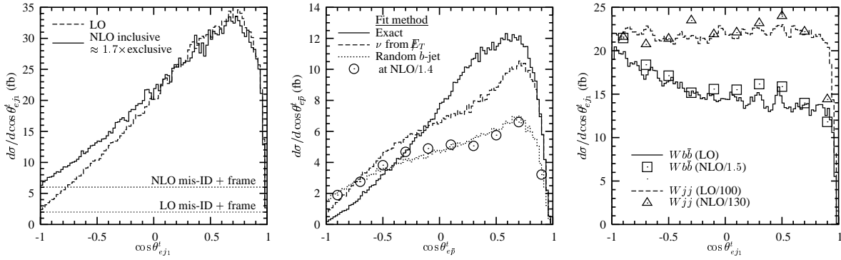
Fig. 3.2.44: Cosine of angle ( \cos \theta_{e j_1}^t ) between the charged lepton and the highest- E_T light-quark jet in the top-quark rest frame for (left) t -channel single-top-quark production, and (right) W j j production at the Tevatron. (Center) cosine of angle between the lepton and antiproton for s -channel single-top-quark production.
