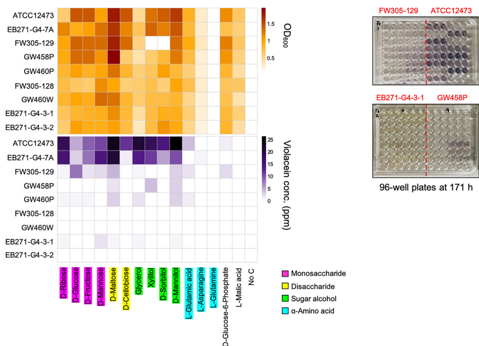
FIG 3 Optical density ( OD_{600} ) and violacein production by nine Janthinobacterium strains grown in 96-well plates with 15 different carbon sources. For each strain, OD_{600} is the highest value measured during the incubation period, and the violacein concentration is also the highest from the three sampling time points (50, 92, and 171 h). The OD_{600} and violacein concentration data are mean values of three replicates.
