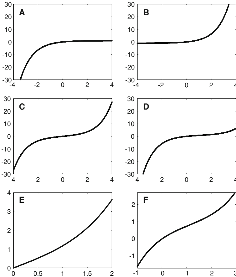
Fig. 1 Panel a U = 1 - x^{-\alpha x} ( \alpha = 1 ); Panel b U = e^{\beta x} - 1 ( \beta = 1 ). Panel c Average of Panels a and b . Panel d \frac{1}{2} average of Panels a and b . Panel e Zoom in on region near x = 0 of Panel c . Panel f Zoom in on region near x = 1.1 , the inflexion point, of Panel d
