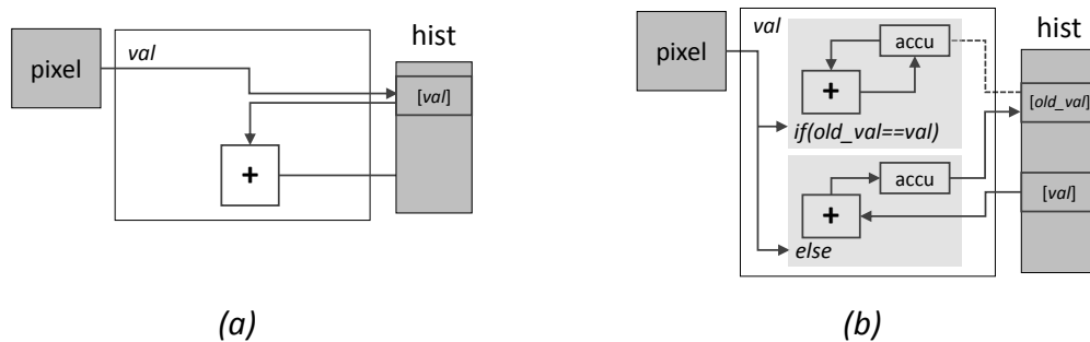
Figure 5.7. Hardware architectures created by software code versus hardware architectures created by restructured code for prefix sum.
