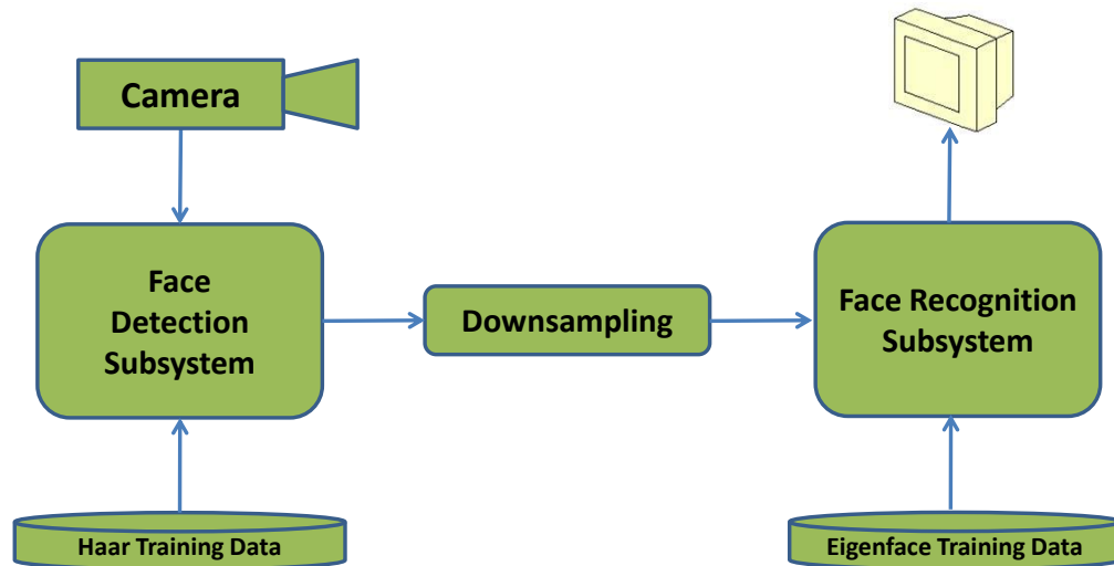
Figure 3.1. Overview of our complete face recognition system on an FPGA. Video data is received from the camera and sent to the face detection subsystem which finds location of the face(s). These face(s) can be in any size; the face detection subsystem looks for faces in a sliding window starting at 20 \times 20 and going all the way to the size of the frame. The architecture then performs downsampling of the detected face to 20 \times 20 , and sends these 400 pixel values to the recognition subsystem. The face recognition subsystem identifies the person and sends the name of the person to the display.
