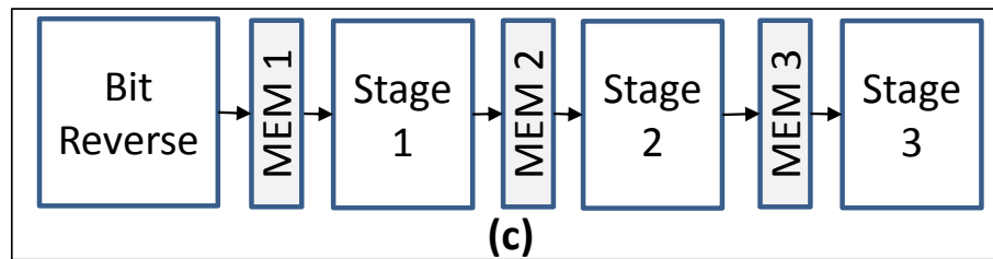
Figure 5.16. Block diagram of FFT
