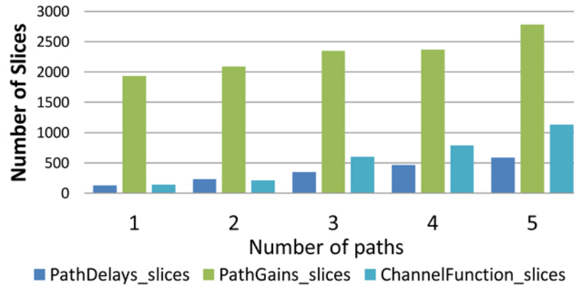
Figure 2.9. Slice numbers for scaling number of paths
