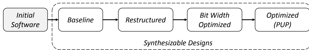
Figure 2.1. Overview of HLS design flow
