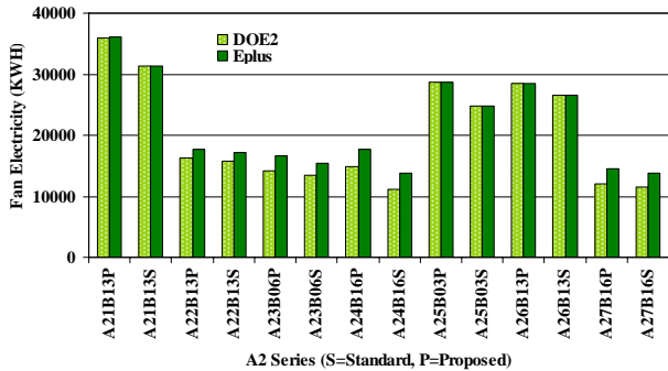
Figure 3. A2 Series Exterior Opaque Envelope Tests Ventilation Fans
