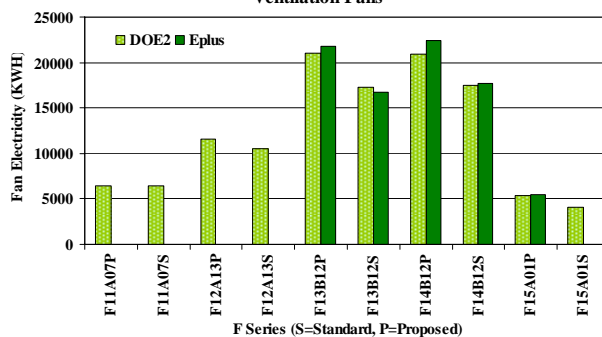
Figure 15. F Series HVAC System Tests Ventilation Fans
