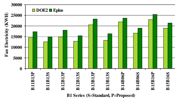
Figure 6. B1 Series Window-to-Wall Ratio Tests Ventilation Fans
