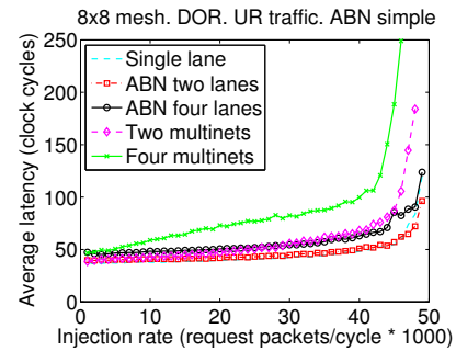
Figure 10: Scaling of ABNs and multinets with UR traffic.
