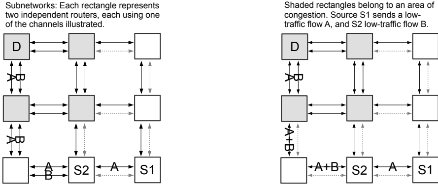
Figure 1: With subnets (left), because flows A and B should be placed in separate resources in high-traffic regions (shaded routers), they are forced to use separate resources in low-traffic regions with multiple and independent subnets. In an ABN (right), packets are free to share resources in low utilization regions. Shaded channels are inactive.
