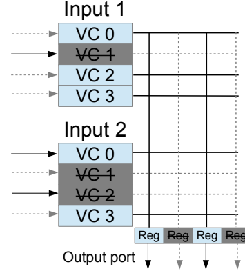
Figure 3: Only two inputs and one output are shown. The switch connects to each VC and each output lane. Those connections are power gated according to the state of the VCs and output lanes, as shown.
