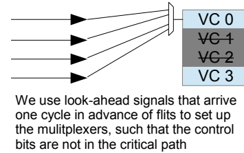
Figure 4: A multiplexer for each VC is required because flits from any lane may be destined to any VC.
