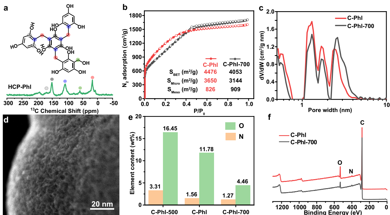
Fig. 2 | Physicochemical characterizations of HCP-Phl, C-Phl, and C-Phl-700. a 13 C{ 1 H} CP/MAS NMR of HCP-Phl. b N 2 adsorption-desorption isotherms of C-Phl and C-Phl-700 at 77 K. c NLDFT pore distributions of C-Phl and C-Phl-700. d STEM
