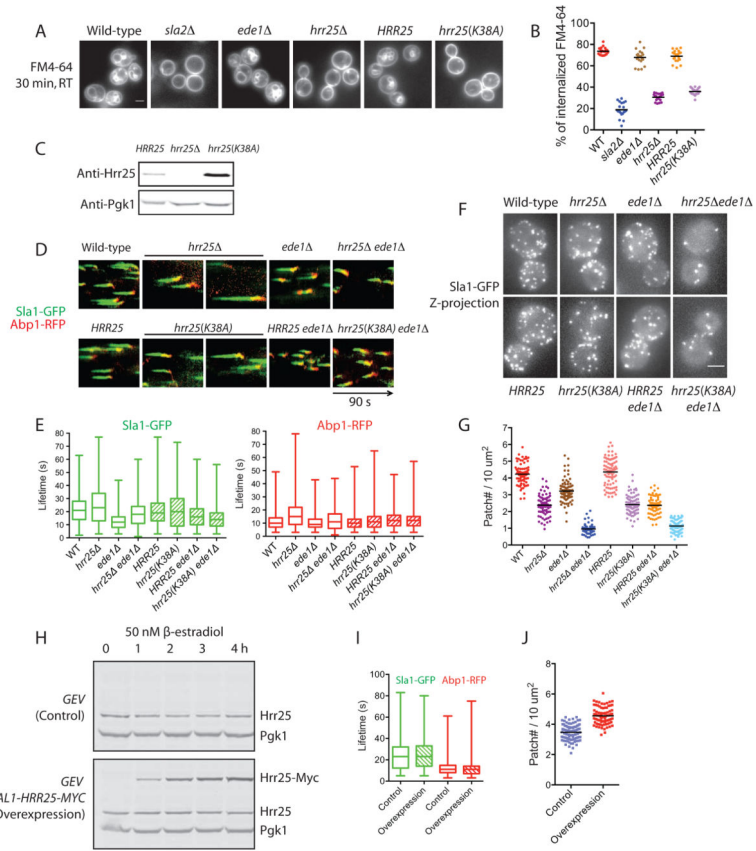
Figure 2. Loss of Hrr25 or its kinase activity results in formation of fewer endocytic sites, whereas Hrr25 overexpression increases the number of endocytic sites formed (A) Wild-type and mutant cells were incubated with FM4-64 for 5 min and chased with fresh media for 30 min at RT. HRR25 is the isogenic wild-type strain for hrr25(K38A) . (B) Percentages for internalized FM4-64 fluorescence intensity relative to whole cell FM4-64 fluorescence intensity are presented. 20 cells were scored for each strain and mean values are presented as black bars. (C) Cell extracts prepared from the indicated strains were analyzed by immunoblotting. (D) Simultaneous two-color imaging of medial focal planes of wild-type and mutant cells expressing Sla1-GFP and Abp1-RFP was performed continuously for 90 s. Representative kymographs are presented. (E) Lifetimes of Sla1-GFP and Abp1-RFP in wild-type and mutant cells. More than 300 Sla1-GFP or Abp1-RFP patches were tracked. Mean values and standard deviations (boxes) are presented. Whiskers indicate the minimum and maximum duration times. (F) Maximum Z-projection of Sla1-GFP patches in wild-type and mutant cells. (G) Quantification of Sla1-GFP patch numbers in wild-type and mutant cells. Sla1-GFP patches in unbudded or large-budded cells were scored using Icy software. The area used to calculate the patch density was the area of a sphere of the same radius as the circle on which all of the patches of the 3-D cell were projected for the maximum intensity. Averages (black bars) of more than 50 cells for each strain are presented. (H) Cells harboring either GEV (control) or GEV P GAL -HRR25-MYC (Hrr25 overexpression) were grown to log phase, induced with 50 nM \beta -estradiol, and harvested at the indicated time points. Whole cell extracts were subjected to immunoblotting. Intensity of total Hrr25 (endogenous Hrr25 and overexpressed Hrr25-Myc)
