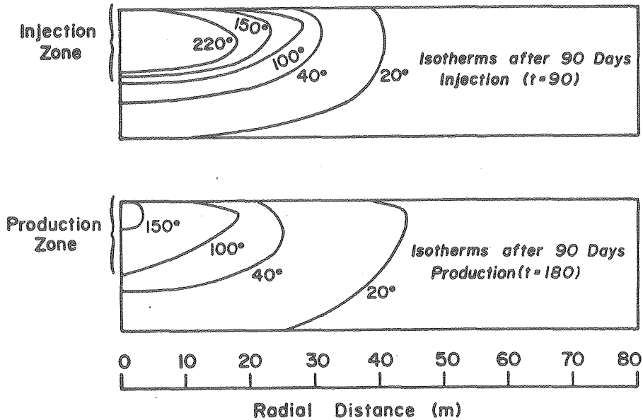
Figure 11. Calculated isotherms for partial penetration after 90-day injection and production periods in the first cycle. (Tsang et al., 1978)
