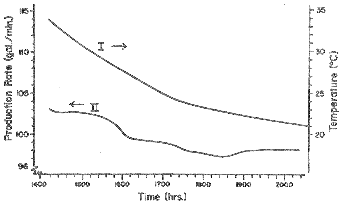
Figure 6. Experiment by Auburn University - temperature curve (curve I) and production flow rate (curve II) as functions of time during the recovery portion of the experiment (Warren, Molz, and Jones, 1977)
