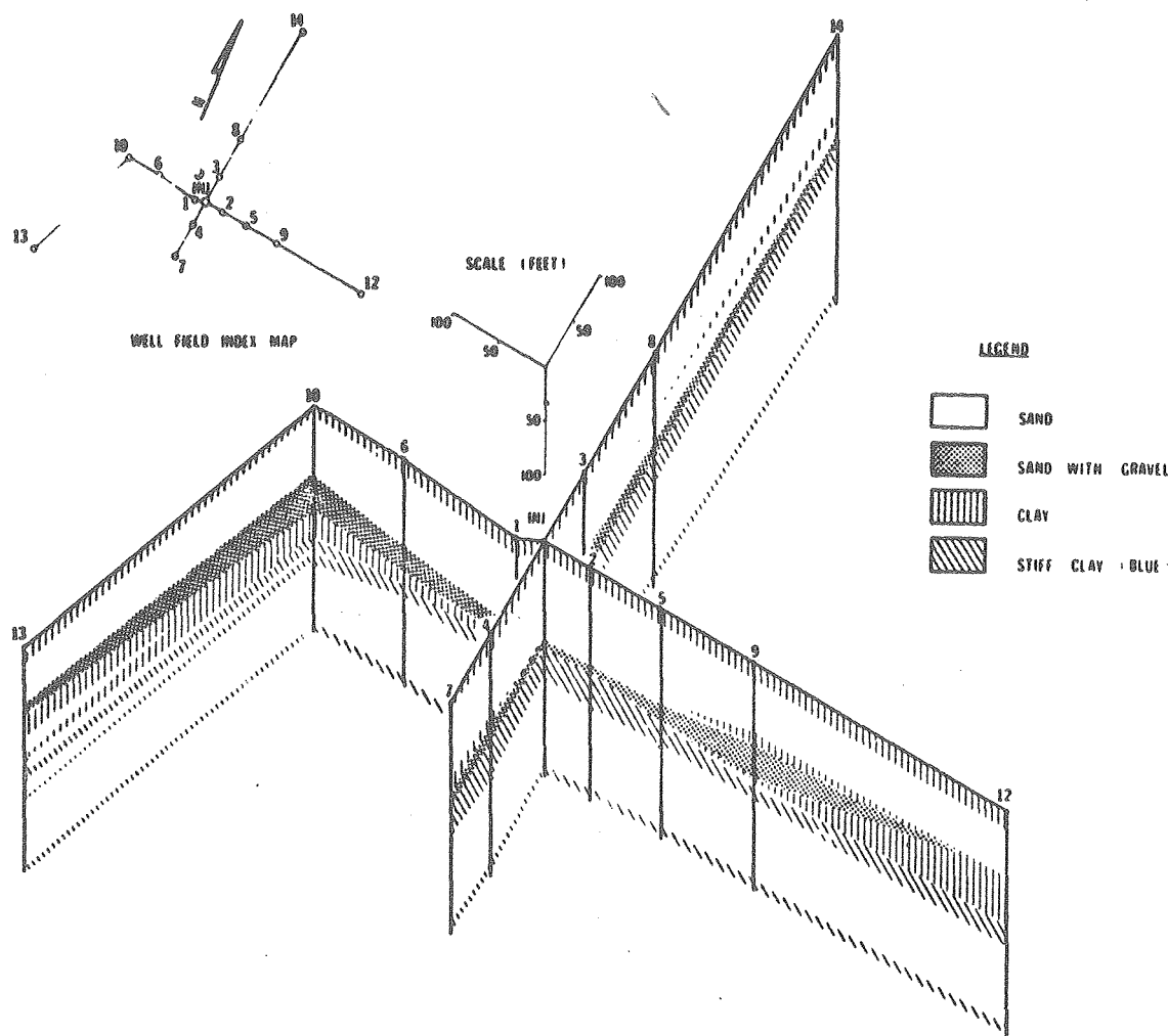
Figure 5. Experiment by Auburn University - fence diagram of the experimental well field; the injection well is labeled INJ. (Molz and Warman, 1978)
