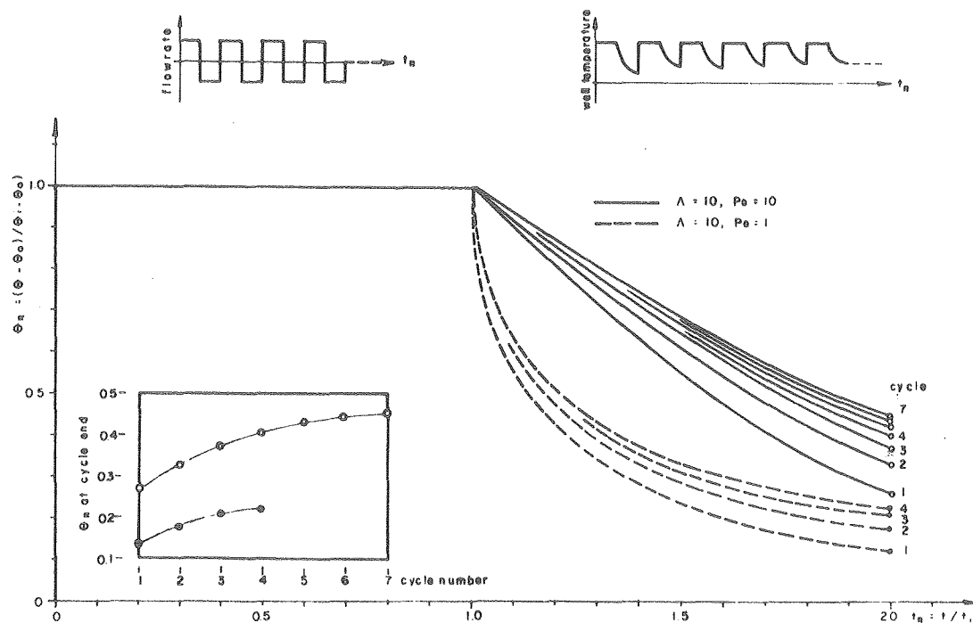
Temperatures evolution at central well during successive cycles of hot water injection and production. Consequences of \tilde{\lambda} = 10, \lambda ( Pe = 1 instead of 10).
