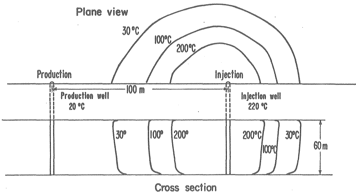
Figure 12. Calculated isotherms for a two-well system after 90 days of injection; plane and cross section views. (Tsang et al., 1978)
