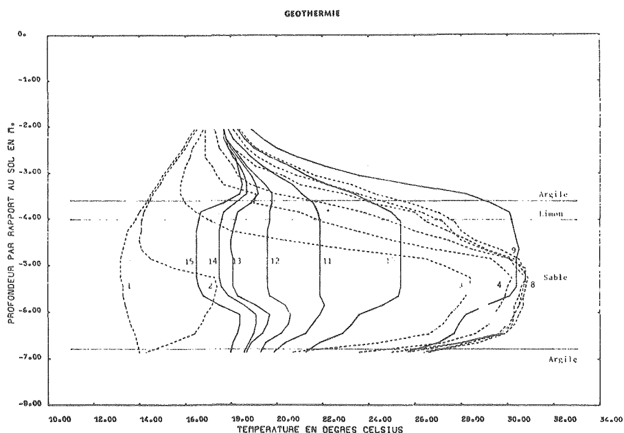
Figure 3. Bonnaud experiment (first cycle) - temperature log in well P2 for the period August 12-14, 1977. (Fabris and Gringarten, 1977)
